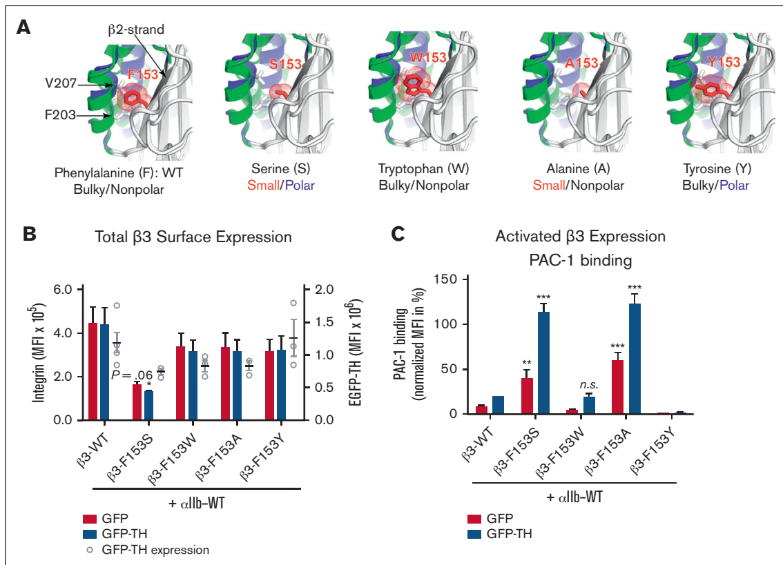
Figure 6. Expression analysis of several mutants suggests that 153aa of \beta 3 with a bulky aromatic and nonpolar structure can maintain normal integrin expression and function. (A) In silico mutagenesis of F153 \beta 3 with small and bulky amino acid shows the space filling effect of the sidechain volumes. The F153S and F153A mutations may render \alpha IIb \beta 3 constitutively active by facilitating an unrestricted inward movement of \alpha 2-helix during the conformational transition of the \beta 3 integrin from a resting to an active state, whereas the F153W and F153Y may limit such movement. In silico mutagenesis were made in PyMol using PDB 2vdo and 3fcs. The resting and active conformations of \alpha 2-helix are highlighted in green and blue, respectively. (B) Immunofluorescent cytometric analysis to quantitate MFI expression levels of transgenic mutant \beta 3-integrin on the surface of HEK293FT. Integrin \alpha IIb and mutated \beta 3 subunits plus GFP or GFP-TH (talins-head integrin activation construct) were cotransfected into HEK293FT cells. Harvested cells were then labeled with an anti- \beta 3 mAb (AP3). GFP immunofluorescence was used as a control for transfection efficiency and integrin double-positive cells were analyzed for their MFI of either AP3 or GFP by immunocytometry. Results show that there is a significant reduction in the cell surface integrin expression of GT mutation ( \beta -F153S) compared with the WT control ( \beta -WT) whereas there is no statistical significance in total \beta 3 surface expression between the WT and the other \beta 3 variants (F153W, F153A, and F153Y). Data are presented as mean MFI + SEM ( n \geq 3 ) and unpaired 2-tailed Student t test was performed to compare the mutants with WT under the same condition or as indicated ( P = .06 ). (C) Maximum integrin activity after stimulation with GFP-TH is detected by the binding of PAC-1, which is specific for the active conformation of \alpha IIb \beta 3. Integrin \alpha IIb and indicated \beta 3 subunits plus GFP or GFP-TH are cotransfected into HEK293FT cells. Integrin and GFP double-positive cells were analyzed for the PAC-1 binding via immunocytometry. PAC-1 binding was quantified and normalized to the total integrin expression showing that (1) bulky aromatic, nonpolar (F,W) are activated identically; (2) bulky aromatic polar (Y) activation is negatively disrupted; and (3) small, polar and nonpolar side-chains (S,A) place \alpha IIb \beta 3 in a constitutively activate confirmation without (red bar) or with (blue bar) talin head domain present. PAC-1 binding is normalized to the total integrin expression. Data are presented as MFI in percentage + SEM ( n \geq 3 ) and unpaired 2-tailed Student t test was performed to compare the mutants with WT under the same condition or as indicated. * P < .05 , ** P < .01 , *** P < .001 . n.s., not significant.
