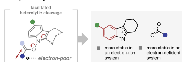
Fig. 9 Mechanistic rationale of the IHT reaction. (A) Electronic responsiveness of the system in a concerted pathway; (B) electronic responsiveness of the system in a dissociative pathway.
