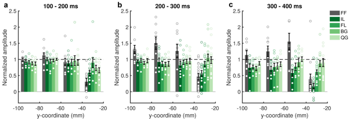
Extended Data Figure 2. Spatiotemporal mapping of selectivity to hierarchical orthographic stimuli. Word-amplitude normalized selectivity profiles grouped in 20 mm intervals along the y (antero-posterior) axis in Talairach space for three consecutive time windows (20 patients).
