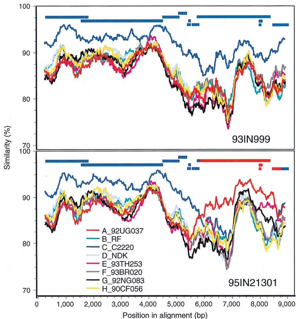
FIG. 1. Plots of similarity (generated by SimPlot) of a set of reference sequences to the 93IN999 (upper panel) and 95IN21301 (lower panel) genomes. Each curve is a comparison between the genome being analyzed and a reference genome. Each point plotted is the percent identity within a sliding window 600 bp wide centered on the position plotted, with a step size between points of 20 bp. Positions containing gaps were excluded from the comparison. The horizontal bars above the curves are a cartoon of the open reading frames of the HIV-1 genome, arranged as indicated in Fig. 3. The colors are consistent with those used for the similarity curves and indicate the subtype to which that part of the genome is most similar based on the adjacent similarity plot. Results for the remaining four genomes discussed in this report were consistent with those for 93IN999.
