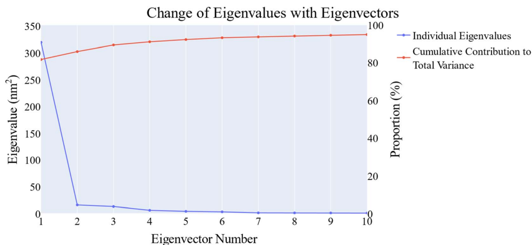
Fig. 16 The change in the eigenvalues with increasing the eigenvectors (blue line) and the cumulative variance retained in the eigenvectors is shown (red line).
