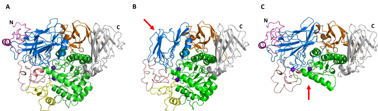
Fig. 2 Models of wild type and mutant human GAA proteins, exons 2–3 and exons 6–10 deleted transcript variants with colored domains. A Structure of wild type GAA. B Structural model of GAA protein containing deletion of exons 2–3. Deletion of exons 2–3 results in the loss of the trefoil type-P domain and some missing \beta -sheets at the N-terminal \beta -sheet domain (indicated by a red arrow). C Structural model of GAA protein containing deletion of exons 6–10. Deletion of exons 6–10 results in some missing parts of the N-terminal \beta -sheet domain and the catalytic GH31 ( \beta/\alpha ) 8 barrel domain, including insert I and some parts of insert II (indicated by a red arrow). Cartoon representation of the structure of GAA consisting of the trefoil type-P domain (residues 81–136) (light magenta), the N-terminal \beta -sheet domain (residues 137–358) (marine), the catalytic GH31 ( \beta/\alpha ) 8 barrel domain (residues 359–720) (green) which consists of insert I (residues 444–492) (yellow) and insert II (residues 522–572) (salmon), the proximal \beta -sheet (residues 721–820) (orange) and distal \beta -sheet (residues 821–952) (grey) domains. Catalytic residues (purple) are depicted as spheres. N N terminus, C C terminus
