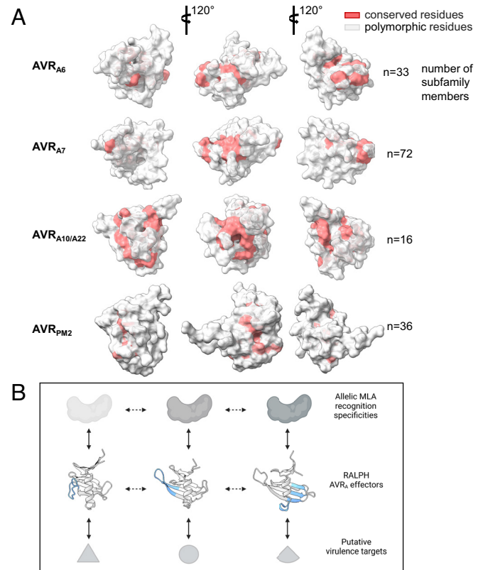
Fig. 5. RALPH effector subfamilies harboring avirulence effectors have overlapping or distinct conserved surface arrays. (A) All CSEPs from B. graminis f sp poae , lolium , avenae , tritici 96224, hordei DH14, secalis S1459, triticales T1-20, and dactylidis were subjected to BLASTP. CSEPs that share >30% sequence identity and that are similar in size to the crystallized RALPH AVR effectors were retained for further analysis using Muscle. Red color indicates conserved (70% threshold) residues. (B) Model for MLA receptor and RALPH AVR A effector coevolution. Major local structural differences between RALPH AVR A effectors are highlighted in blue. Solid bidirectional arrows indicate selection pressure by coevolving protein pairs, dashed bidirectional arrows represent adaptive genetic changes in RALPH effectors.
