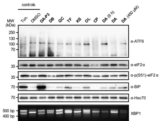
Fig. 5 UPR assessment of HEK293T cells treated with the compounds of interest, the positive control tunicamycin (Tun.), or DMSO (as a vehicle control). Immunoblotting was performed against ATF6, eIF2 \alpha , phosphorylated eIF2 \alpha , BiP or Hsc70. XBP1 splicing was analysed using agarose gel electrophoresis. Cells were treated with 100 \mu M compound for 16 h unless otherwise indicated.
