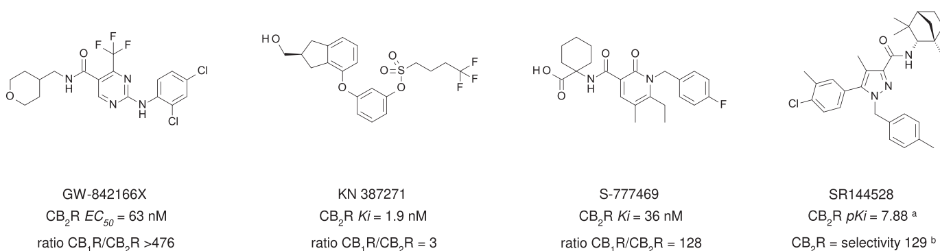
Fig. 20. Chemical structure, CB_2R binding affinity or functional activity, and selectivity of clinically evaluated CB_2R agonists and CB_2R inverse agonists SR144528 containing five- and six-membered central cores. a Consensus human CB_2R binding affinity values from a multicentric collaborative profiling effort between multiple independent academic laboratories and industry (Soethoudt et al., 2017). b CB_2R selectivity ( 10^{(pK_i CB_2R - pK_i CB_1R)} ).
