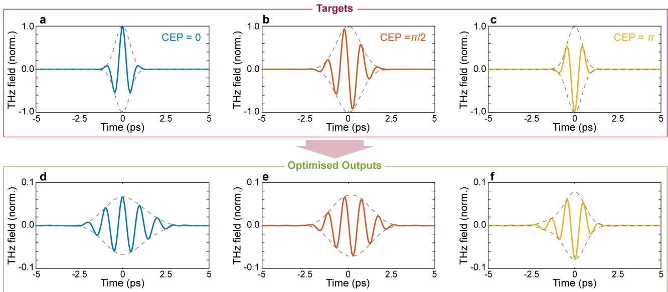
Figure 5. Carrier envelope phase (CEP) modulation. Temporal profiles of target and optimised pulses for CEP \phi = 0 . ( a , d ), \phi = \frac{\pi}{2} ( b , e ), and \phi = \pi ( c , f ). For all cases, the input field is the transform limited pulse shown in Figure 2a. Numerical parameters: spectral correlation \Delta\nu_c = 250 GHz, number of generations 50000, size of population per generation 50.
