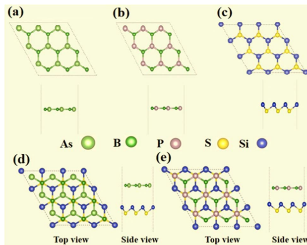
Fig. 1 Top and side views of (a) BA, (b) BP, and (c) SiS monolayers, and (d) BA–SiS and (e) BP–SiS heterobilayers.
