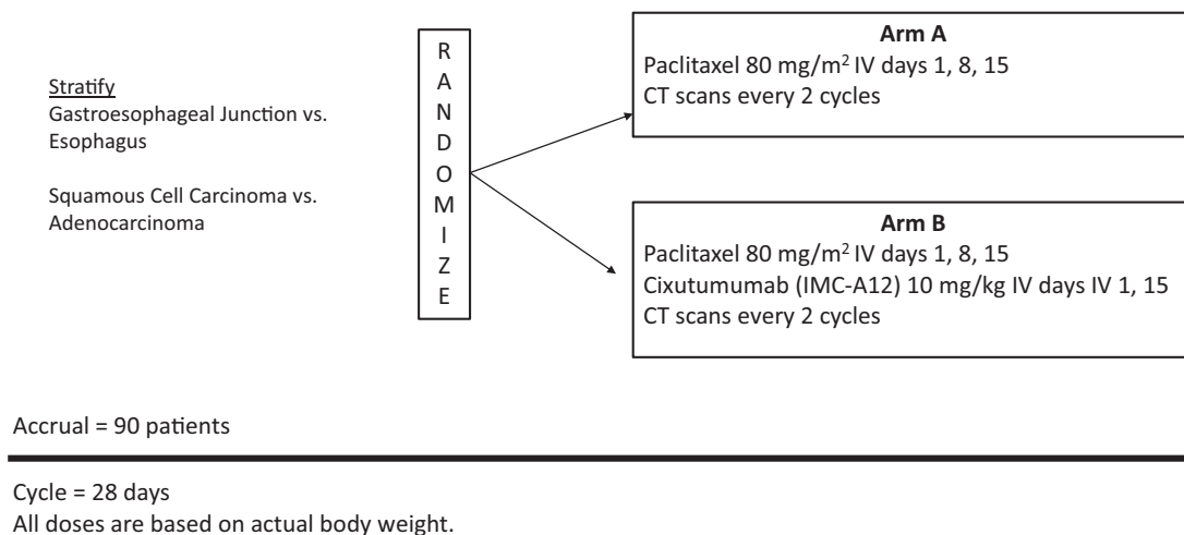
Figure 1. Study schema.
