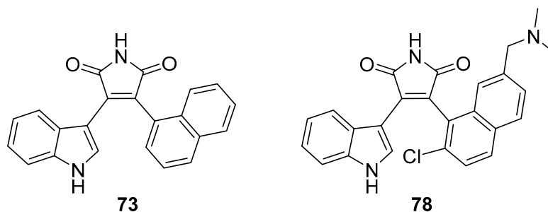
Figure 10. Naphthylindolylmaleimides 73 and 78 .
