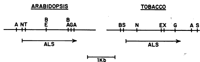
FIG. 1. Restriction enzyme maps of tobacco and Arabidopsis ALS genes. Phage \lambda genomic DNA clones carrying tobacco or Arabidopsis ALS genes were digested with restriction enzymes, fractionated by gel electrophoresis, transferred to filters, and probed with a labeled yeast ALS gene. Maps consistent with the observed fragment sizes were inferred from the data. The sites shown were subsequently confirmed by DNA sequence analysis. A, Ava I; B, Bam HI; E, Eco RI; G, Bgl II; N, Nco I; S, Ssp I; T, Sst II; X, Xba I.
