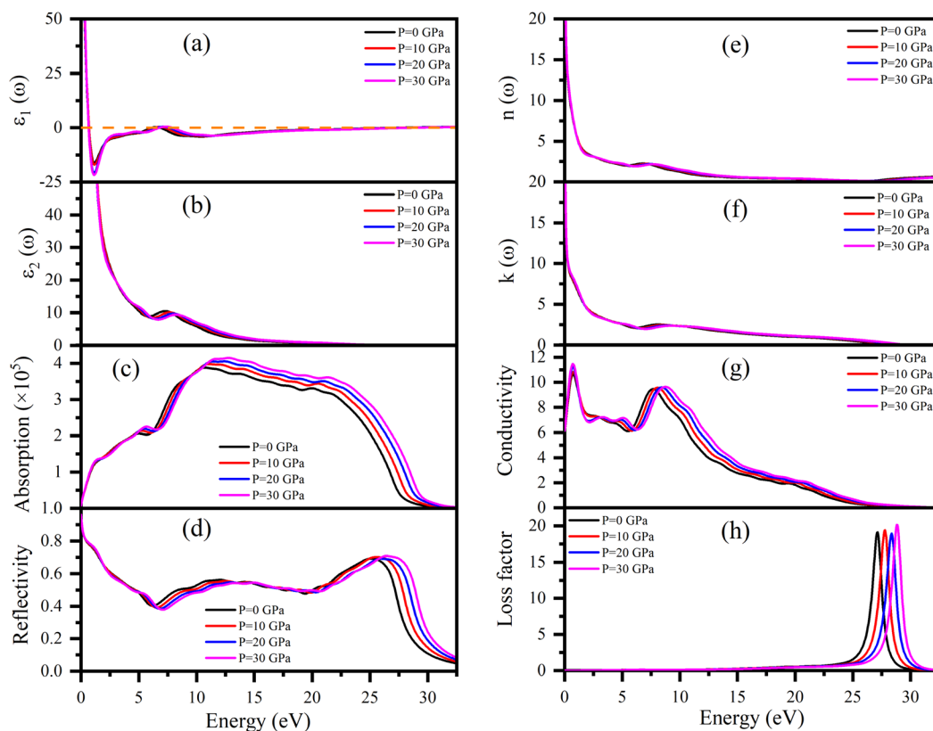
Fig. 11 (a) \varepsilon_1(\omega) , (b) \varepsilon_2(\omega) , (c) absorption coefficient, (d) reflectivity, (e) n(\omega) , (f) k(\omega) , (g) optical conductivity, and (h) energy loss function of \text{Ru}_4\text{Al}_3\text{B}_2 in the [100] direction under pressure from 0–30 GPa as a function of photon energy.
