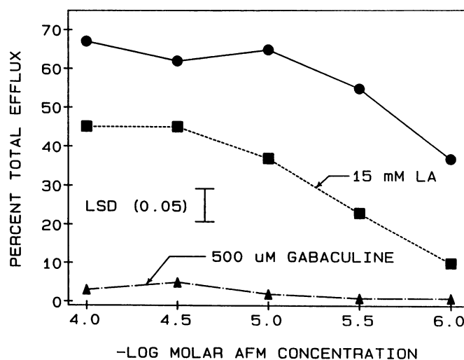
FIG. 8. Effect of inhibitors of porphyrin precursor formation on the membrane-disrupting activity of AFM. After being loaded with 3-O-methyl-D-[ U-^{14}C ]glucose, excised cotyledons were washed under green safelights, placed on media treated with AFM, then held in darkness for 6 h. Inhibitors, 500 \mu M gabaculine ( \blacktriangle — \blacktriangle ) or 15 mM LA ( \blacksquare — \blacksquare ), were added to selected replicates, and all treatments, including AFM alone ( \bullet — \bullet ), were incubated in the dark for a further 10 h. Treatments were then exposed to intermittent illumination (1 min of light in 10 min cycles) for a period of 4 h. Light-activated membrane disruption was induced by placing the treatments under a continuous, high intensity illumination source ( 600 \mu E \cdot m^{-2} \cdot s^{-1} ; PAR) for 3 h. Treatment medium was then recovered and sampled for effluxed radioactivity. Controls and 500 \mu M gabaculine alone showed identical efflux levels of 2%; 15 mM LA alone induced 4% leakage.
