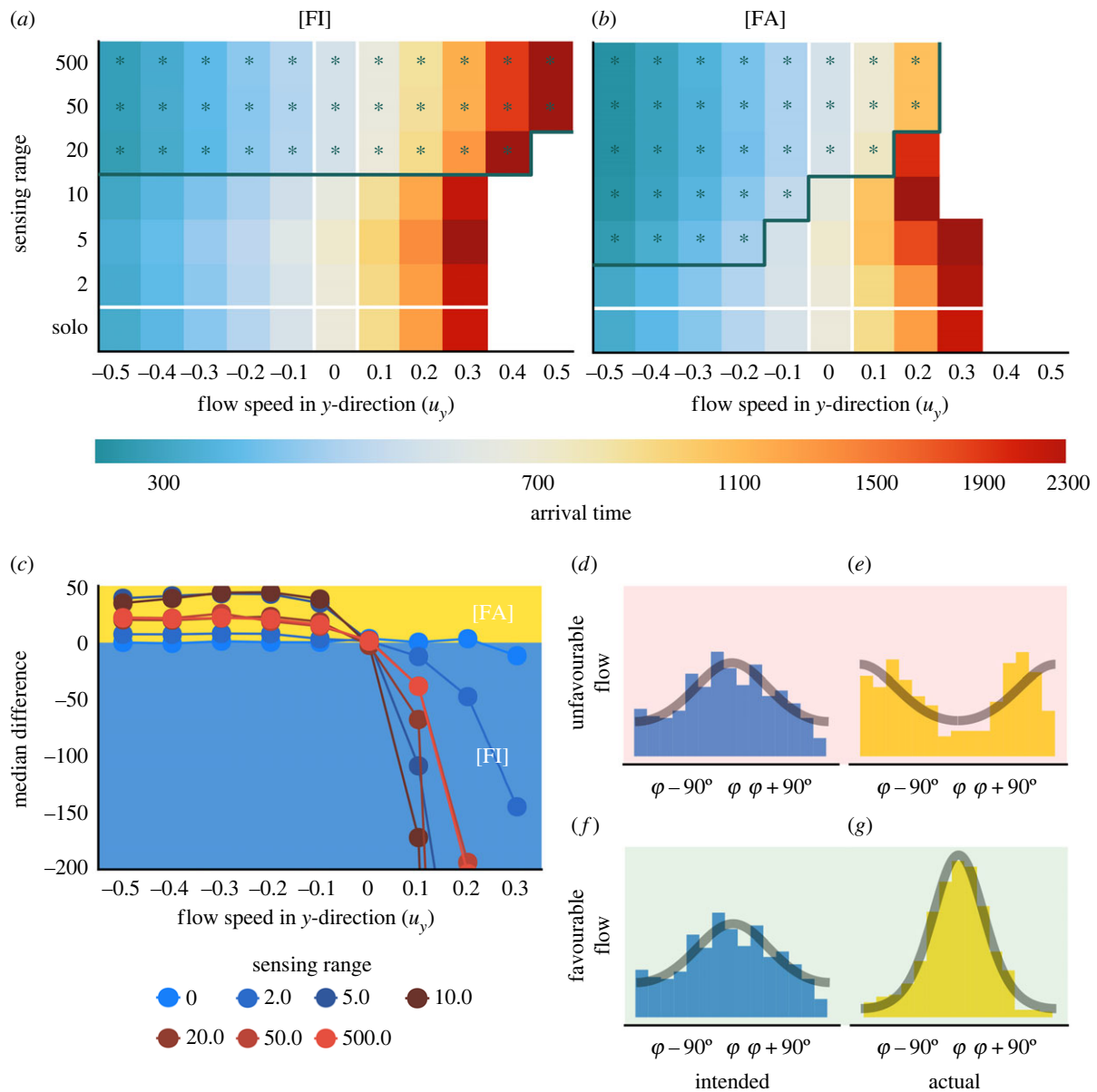
Figure 3. Effect of perception type depends on flow direction. (a,b) Heatmaps of the median arrival time as a function of the flow speed in the y -direction and sensing range. Each parameter combination is averaged over 50 realizations. (a) Results for a fixed range interaction and intended headings [FI]. (b) fixed range interaction and actual headings [FA]. Green asterisks denote parameters where solo navigation was outperformed by \geq 5\% . The green solid line indicates the boundary of the region where collective navigation induces a \geq 5\% improvement. Missing cells indicate where there is failed migration. (c) The difference in median arrival time between the [FI] and [FA] models across a variety of flow strengths and sensing ranges. Positive values (yellow) indicate scenarios in which sharing actual headings leads to faster arrival times than when sharing intended headings (blue). (d–g) Illustrative neighbour heading distributions relative to the goal direction \phi in unfavourable (d,e) and favourable (f,g) flows.
