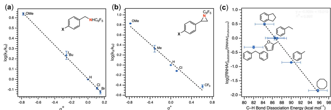
Fig. 4 (a) Intermolecular competition Hammett amination with neat equimolar toluene and para -substituted toluene substrates with ( ^{ArF}L )Cu ( 4 ). (b) Intermolecular competition Hammett aziridination with equimolar styrene and para -substituted styrene substrates in C_6D_6 . (c) Competition amination experiments in neat equimolar ethylbenzene and substrate.
