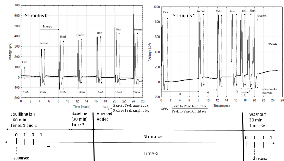
Figure 10. Outline of the experiment. The top part of the figure shows the two different stimulus sets used with the first, keeping the interstimulus interval at 4 ms and increasing the stimulus current. The second maintains a constant stimulus current but gradually shortens the interstimulus interval. The lower graph shows an outline of each experiment and the fact that stimulus set 0 is delivered first followed by stimulus set 1 every 200 ms during the experiment. It also shows the initial equilibration period and the time that the amyloid is added into the fluid, bathing the nerve.
