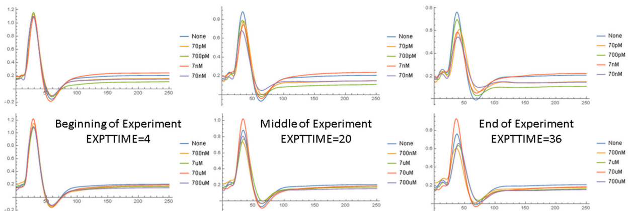
Figure 5. Normalized NAP waveforms averaged over all nerves in same A \beta 42 concentration category at the beginning of the experiment, middle of the experiment, and end of the experiment for the long (166 ms) inter-stimulus interval at different concentrations of A \beta 42. Each curve represents a different concentration of A \beta 42 and “none” is the control case in which no A \beta 42 is added.
