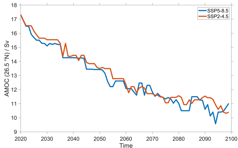
Figure 14 Changes in Atlantic Meridional Overturning Circulation (AMOC) strength over time for SSP5-8.5 and SSP2-4.5. Volumetric flow rate in Sverdrup of the Atlantic Meridional Overturning Circulation (AMOC) derived in the CESM2 for two different climate scenarios for SSP5-8.5 (in blue) and SSP2-4.5 (in red) at 26.5^{\circ} N. The model data have been smoothed using a 5-year moving median.
