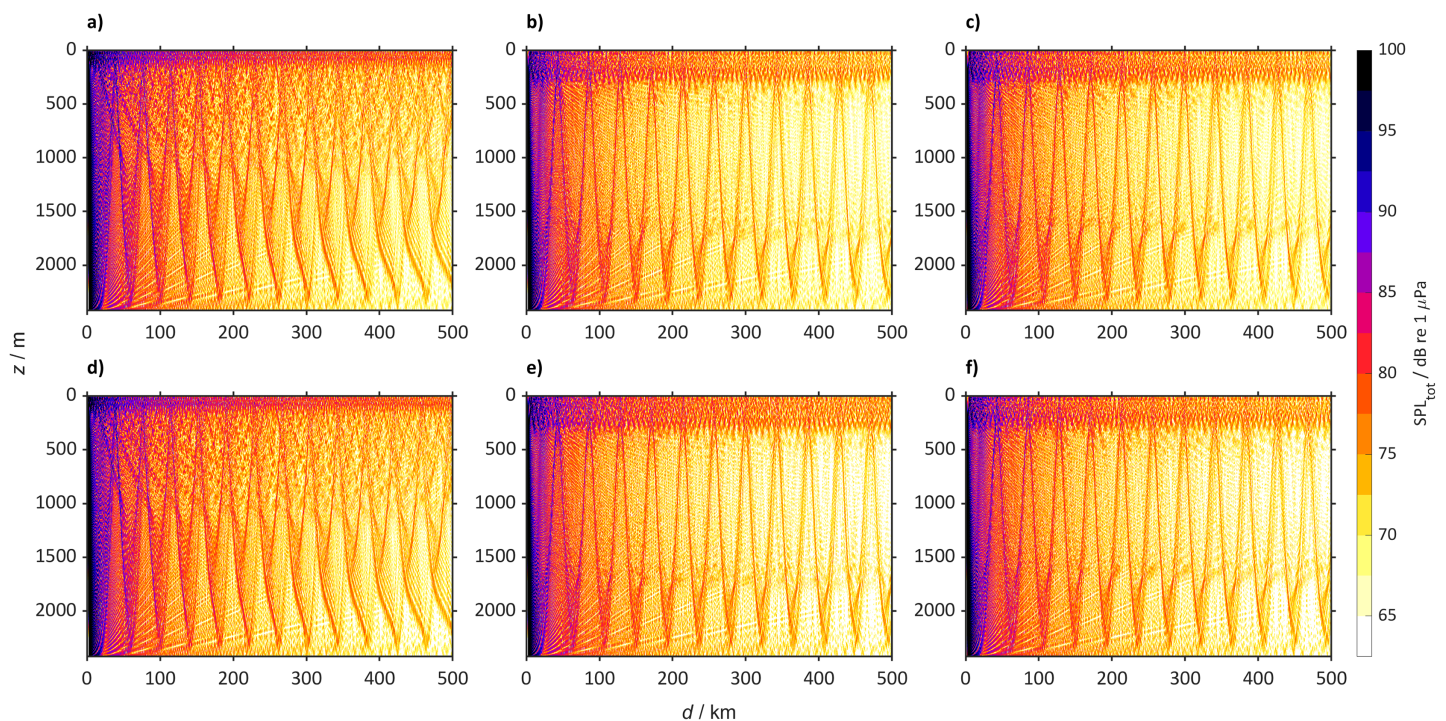
Figure 10 Predicted SPL_{tot} for the Norwegian Sea ( 72^{\circ} N 1^{\circ} W) from a single bulker and wind. Predicted SPL_{tot} for the Norwegian Sea ( 72^{\circ} N 1^{\circ} W) from a single bulker and wind where (A) is winter (2018 to 2022), (B) winter (2094 to 2099) for SSP2-4.5, (C) winter (2094 to 2098) for SSP5-8.5 (D) summer (2018 to 2022), (E) summer (2094 to 2098) for SSP2-4.5 and (F) summer (2094 to 2098) for SSP5-8.5.
