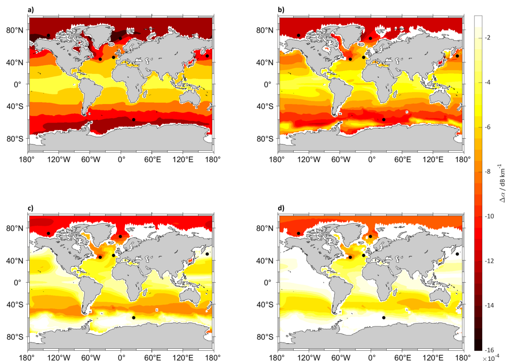
Figure 4 Absorption difference between (2018 to 2022) and (2094 to 2098) for SSP5-8.5. Maps of the difference in 5 years mean of sound absorption ( \alpha ) in \text{dB km}^{-1} in (2094 to 2098) and (2018 to 2022), calculated using van Moll, Ainslie & van Vossen (2009) algorithm at (A) 5, (B) 125, (C) 300 and (D) 640 m depth calculated for SSP5-8.5. The black dots indicate the sound source locations.
