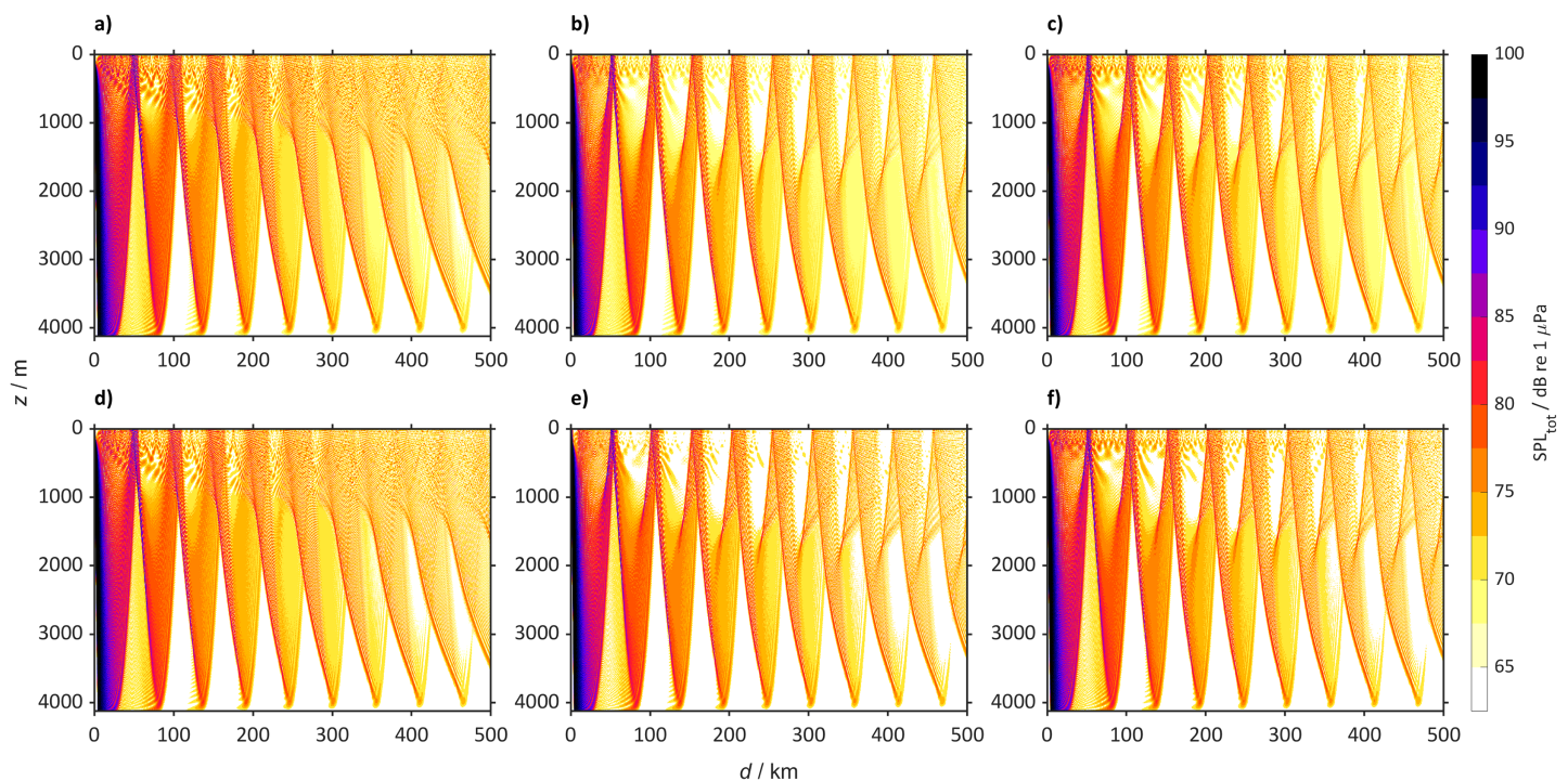
Figure 11 Predicted sound pressure level for the North Pacific Ocean ( 50^{\circ} N 167^{\circ} E) from a single bulker and wind. Predicted SPL_{tot} for the North Pacific Ocean ( 50^{\circ} N 167^{\circ} E) from a single bulker and wind where (A) is winter (2018 to 2022), (B) winter (2094 to 2098) for SSP2-4.5, (C) winter (2094 to 2098) for SSP5-8.5 (D) summer (2018 to 2022), (E) summer (2094 to 2098) for SSP2-4.5 and (F) summer (2094 to 2098) for SSP5-8.5. Full-size DOI: 10.7717/peerj.16208/fig-11
