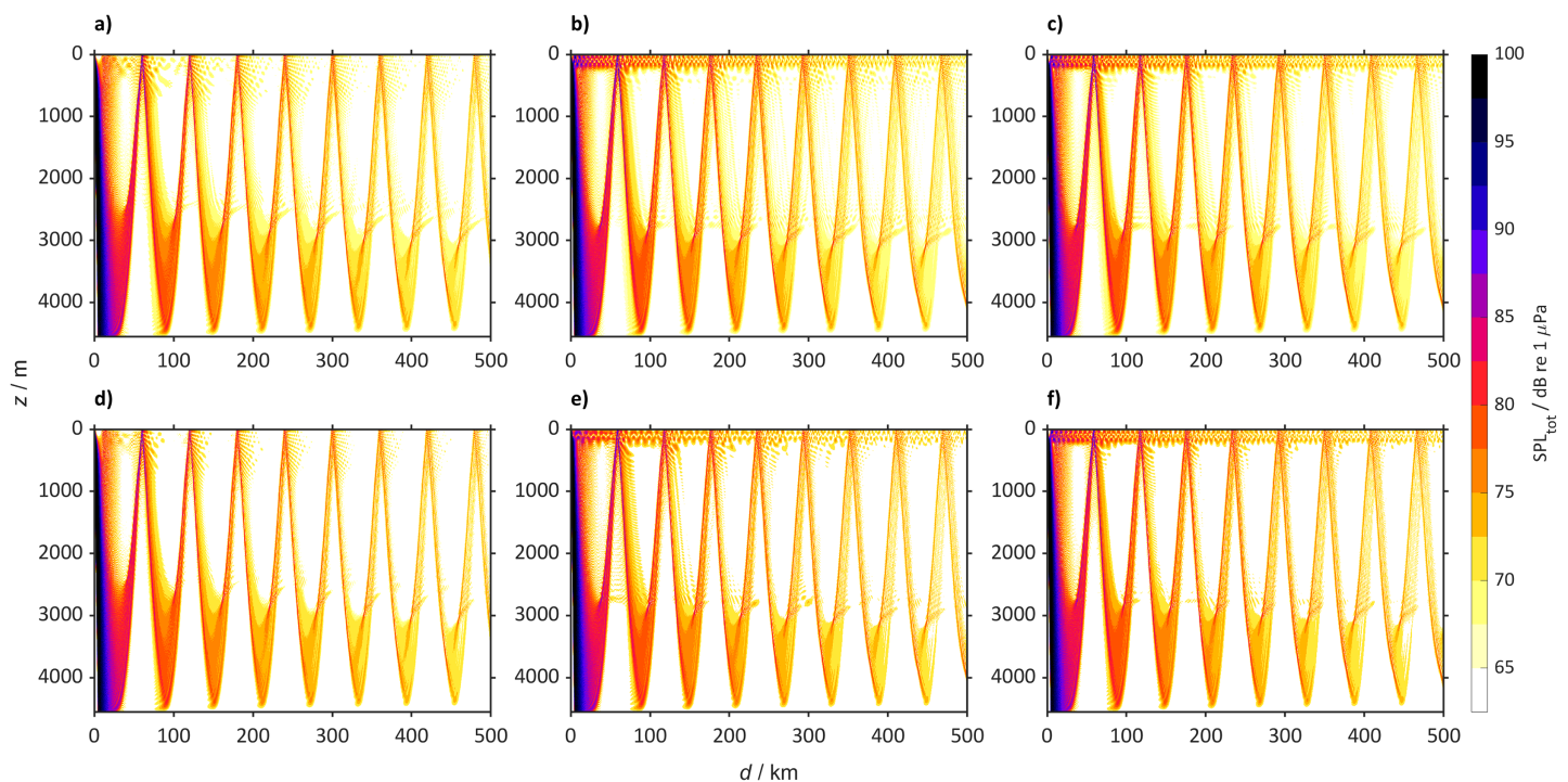
Figure 9 Predicted SPL_{tot} for the Northeast Atlantic Ocean ( 47^{\circ} N 14^{\circ} W) from a single bulker and wind. Predicted SPL_{tot} for the Northeast Atlantic Ocean ( 47^{\circ} N 14^{\circ} W) from a single bulker and wind where (A) is winter (2018 to 2022), (B) winter (2094 to 2098) for SSP2-4.5, (C) winter (2094 to 2098) for SSP5-8.5 (D) summer (2018 to 2022), (E) summer (2094 to 2098) for SSP2-4.5 and (F) summer (2094 to 2098) for SSP5-8.5.
