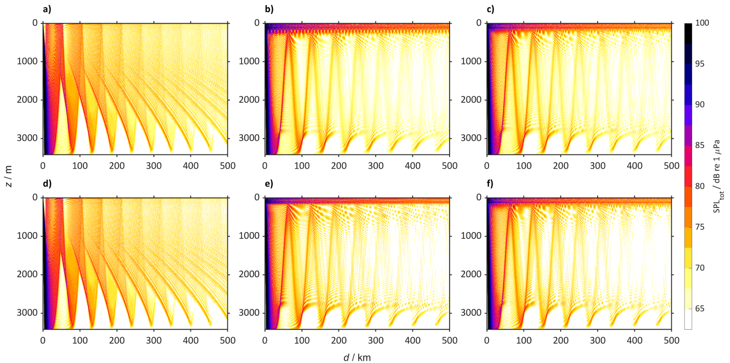
Figure 7 Predicted SPL_{tot} for the Northwest Atlantic Ocean ( 45^{\circ} N 40^{\circ} W) from a single bulker and wind. Predicted SPL_{tot} for the Northwest Atlantic Ocean ( 45^{\circ} N 40^{\circ} W) from a single bulker and wind where (A) is winter (2018 to 2022), (B) winter (2094 to 2099) for SSP2-4.5, (C) winter (2094 to 2098) for SSP5-8.5 (D) summer (2018 to 2022), (E) summer (2094 to 2098) for SSP2-4.5 and (F) summer (2094 to 2098) for SSP5-8.5.
