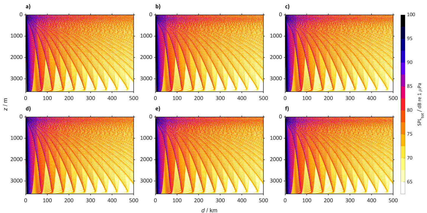
Figure 12 Predicted sound pressure level for the Arctic Ocean (75° N 140° W) from a single bulker and wind. Predicted SPL_{tot} for the Arctic Ocean (75° N 140° W) from a single bulker and wind where (A) is winter (2018 to 2022), (B) winter (2094 to 2098) for SSP2-4.5, (C) winter (2094 to 2098) for SSP5-8.5 (D) summer (2018 to 2022), (E) summer (2094 to 2098) for SSP2-4.5 and (F) summer (2094 to 2098) for SSP5-8.5.
