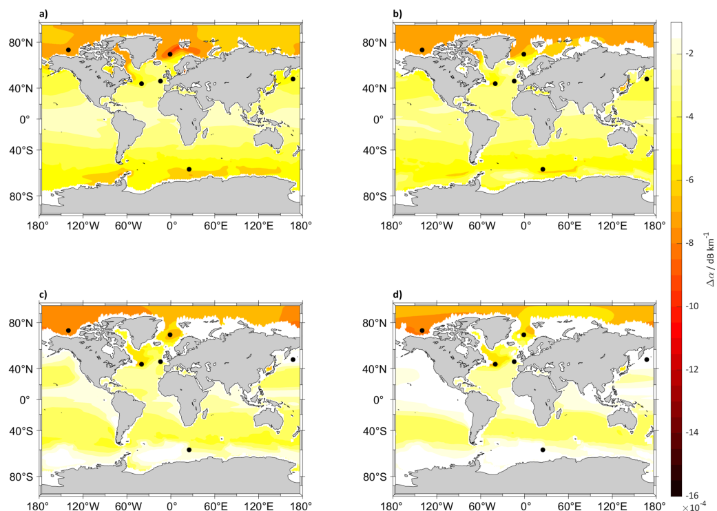
Figure 5 Absorption difference between (2018 to 2022) and (2094 to 2098) for SSP2-4.5. Maps of the difference in 5 years mean of sound absorption ( \alpha ) in \text{dB km}^{-1} in (2094 to 2098) and (2018 to 2022), calculated using van Moll, Ainslie & van Vossen (2009) algorithm at (A) 5, (B) 125, (C) 300 and (D) 640 m depth calculated for SSP2-4.5. The black dots indicate the sound source locations.
