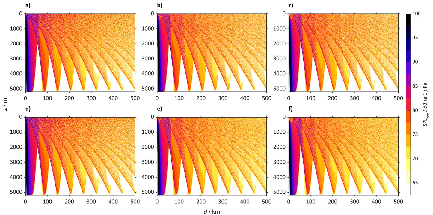
Figure 13 Predicted sound pressure level for the Southern Ocean ( 60^{\circ} S 25^{\circ} E) from a single bulker and wind. Predicted SPL_{tot} for the Southern Ocean ( 60^{\circ} S 25^{\circ} E) from a single bulker and wind where (A) is winter (2018 to 2022), (B) winter (2094 to 2099) for SSP2-4.5, (C) winter (2094 to 2098) for SSP5-8.5 (D) summer (2018 to 2022), (E) summer (2094 to 2098) for SSP2-4.5 and (F) summer (2094 to 2098) for SSP5-8.5.
