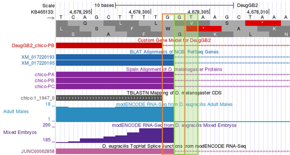
Figure 10. Use of incorrect splice site (GG) in the annotation of the chico ortholog in D. eugracilis . Extending the end of the proposed coding exon by one nucleotide (to 4,678,302) will utilize the canonical splice donor site (GT) and is more consistent with the available gene predictions and RNA-Seq data. The revised coding exon coordinate is supported by the splice junction prediction JUNC00062858 (score = 216).
