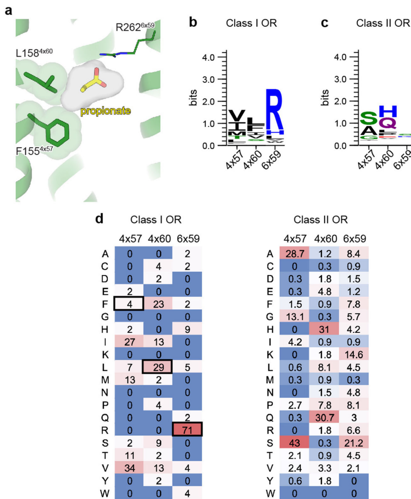
Extended Data Figure 6. Conservation of residues within the odorant binding pocket. a) View of propionate-contacting residues. Conservation weblog of key residues in Class I (b) and Class II ORs (c) . d) The percentage of receptors harboring a given amino acid at each position are shown for all human Class I and Class II ORs. OR51E2 residues at each position are indicated by a black box.
