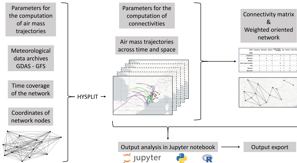
Figure 1. Simplified architecture of tropolink. After providing input parameters, dates, and node locations, HYSPLIT is executed using open meteorological data archives to generate sets of trajectories. Subsequently, connectivities between sites resulting from these trajectory sets can be computed by specifying connectivity parameters. Sets of trajectories and connectivities can then be explored within jupyter notebooks embedded in tropolink and exported for publication and in-depth analysis.
