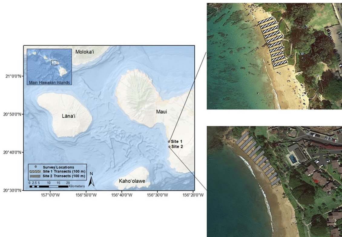
Figure 1. Map showing the location of the two survey sites on Maui with inserts showing the topographic details and locations of the 100 m transects. Site 1: Kama'ole Beach Park III; Site 2: Ulua Beach. Ocean Base Map Source: Esri, GEBCO, NOAA, National Geographic, DeLorme, HERE, Geonames.org, and other contributors 35 .
