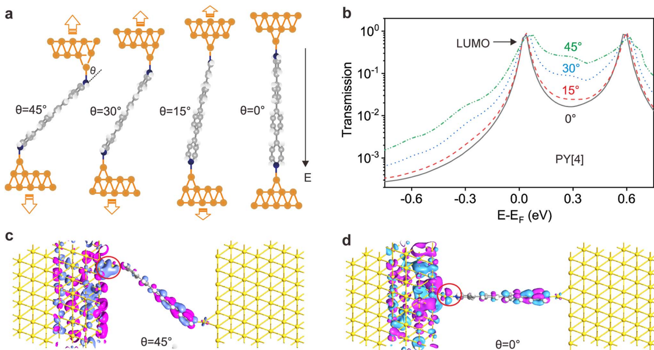
Fig. 5 Transmission characteristics of PY[4] molecular junction with different tilt angles between the nitrogen–gold bond and the pyridine plane ( \pi^* -system). (a) Examples of junction geometries relaxed at different tip–sample distances with different nitrogen–gold bond orientations. (b) Transmission characteristics plotted on the semi-logarithmic scale for the molecular junctions. The green dotted, blue dashed, red dashed and black solid lines denote the angle ( \theta ) between the nitrogen–gold bond and \pi^* -system, which are 45°, 30°, 15° and 0°, respectively. (c) Transmission eigenstates at 0.3 eV of the PY[4] molecular junction with a tilt angle of 45° and (d) 0°. The red circle highlights the transmission eigenstates at the interface.
