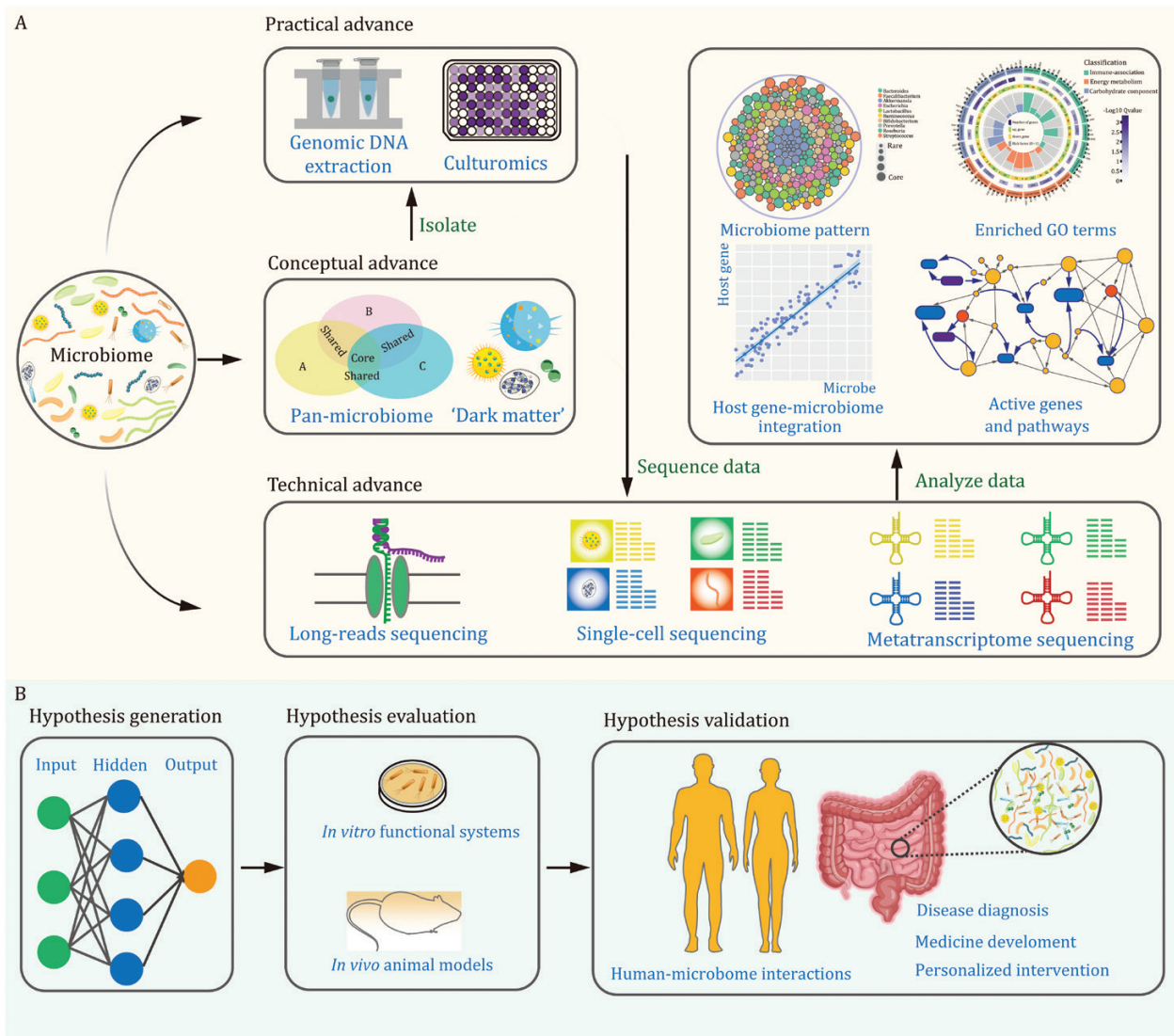
Figure 3. Future direction of microbiome research. (A) The flow chart presents an overview of the practical, conceptual, and technical advances in microbiome for studying its function and mechanisms. (B) The research data of microbiome is essential for hypothesis generation, evaluation, and validation.
