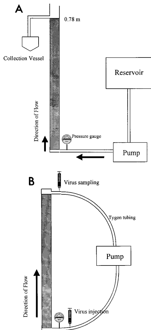
FIG. 1. Schematic diagram of the batch flowthrough column used in the viral batch transport studies. (B) Schematic diagram of the continuous column used in the viral transport studies.
