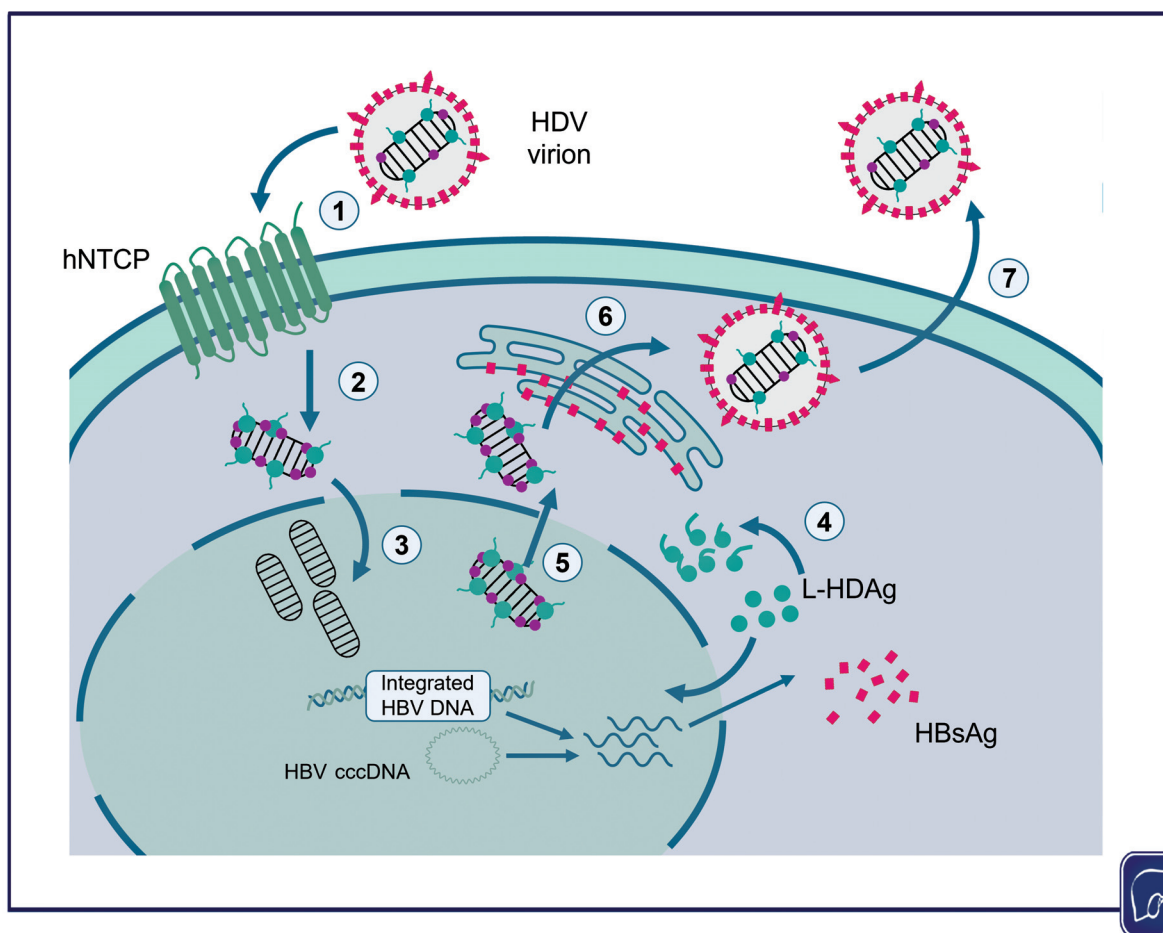
Fig. 3. Life cycle of HDV. (1) The HBsAg envelope of the HDV virion binds to the extracellular loop(s) of the sodium taurocholate cotransporting polypeptides (NTCP) receptor. This receptor, a transmembrane protein and the same receptor HBV uses for entry, mediates the transport of bile acids, removing them from circulation. (2) The binding with NTCP leads to endocytosis and thus the ribonucleoprotein (RNP) complex enters the hepatocyte cytoplasm. (3) This allows the HDV RNP complex to enter the nuclei of hepatocytes, where HDAg mRNA transcription and replication of HDV RNA occur. (4) L-HDAg is farnesylated by a cellular farnesyltransferase before being retranslocated to the nucleus. (5) S- and L-HDAg interact with the newly synthesized genomic RNA to form viral RNP that is exported to the cytoplasm. (6) Viral RNPs interact with the cytosolic part of HBsAg at the endoplasmic reticulum surface inducing their envelopment. (7) HDV virions are then secreted (modified from Sandmann and Cornberg, 2021 98 ). cccDNA, covalently closed circular DNA; HBsAg, hepatitis B surface antigen; HBV, hepatitis B virus; HDV, hepatitis delta virus; hNTCP, human sodium taurocholate cotransporting polypeptide; L-HDAg, large hepatitis D antigen; S-HDAg, small HDAg.
