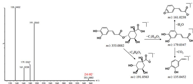
Fig. 6 Mass spectra and possible fragmentation pathway of chlorogenic acid in negative ion mode.
