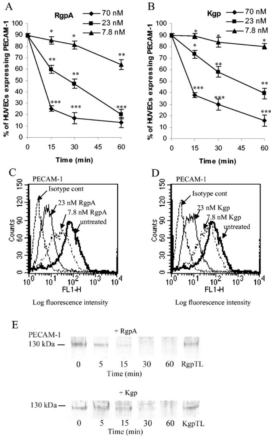
FIG. 2. Decrease of PECAM-1 expression on HUVECs following gingipain treatment. (A and B) Confluent HUVECs were incubated with a 5 mM concentration of cysteine-activated RgpA or Kgp at the indicated concentrations and times without serum for 1 h at 37°C. HUVECs were then harvested by scraping, stained with anti-PECAM-1 or isotype-matched antibody, and measured by flow cytometry. Results are representative of three separate experiments that yielded similar results. Error bars indicate the means \pm SEM. *, P < 0.05 ; **, P < 0.01 ; and ***, P < 0.001 compared with untreated HUVECs. (C and D) Representative FACS profiles of PECAM-1 expression on HUVECs after treatment in the presence or absence of gingipains at indicated concentrations for 1 h. Results are representative of three separate experiments that yielded similar results. (E) Confluent HUVECs were incubated with RgpA or Kgp at a concentration of 70 nM for various times at 37°C under serum-free conditions. Proteolysis was inhibited in aliquots by the addition of 2 mM TLCK. (Endothelial cells were then harvested by scraping, washed with PBS, and lysed directly in SDS reducing sample buffer with 20% (vol/vol) protease inhibitor cocktail. Aliquots were then subjected to SDS-10% polyacrylamide gels and transferred to polyvinylidene difluoride membranes for Western blot analysis with antibody against PECAM-1 as described in Materials and Methods. RgpTL, TLCK-inhibited RgpA; KgpTL, TLCK-inhibited Kgp.
