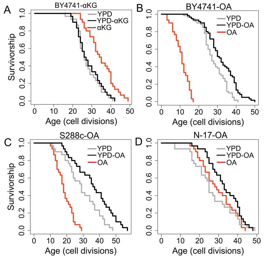
Fig. 7 RLS effect of \alpha -ketoglutarate and orotic acid supplementation. Lifespan curves for cells on medium supplemented with A) \alpha -KG or B), C), D) OA. Standard YPD media contains 2% glucose. YPD- \alpha KG and YPD-OA mediums were prepared by supplementing YPD with 2% \alpha KG or 0.1% OA respectively. \alpha KG and OA mediums contain 2% \alpha KG or 0.1% OA as a carbon source. Lifespan data and the significance of lifespan changes can be found in Supplementary Table 1
