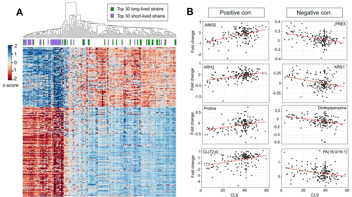
Fig. 2 Selected endophenotypes correlating with CLS. A The heat map on the left panel shows expression patterns of the significantly correlating proteins. Spearman correlation matrix of aggregated protein expression profiles across strains was used for clustering. The top 30 short- and long-lived strains are indi-
