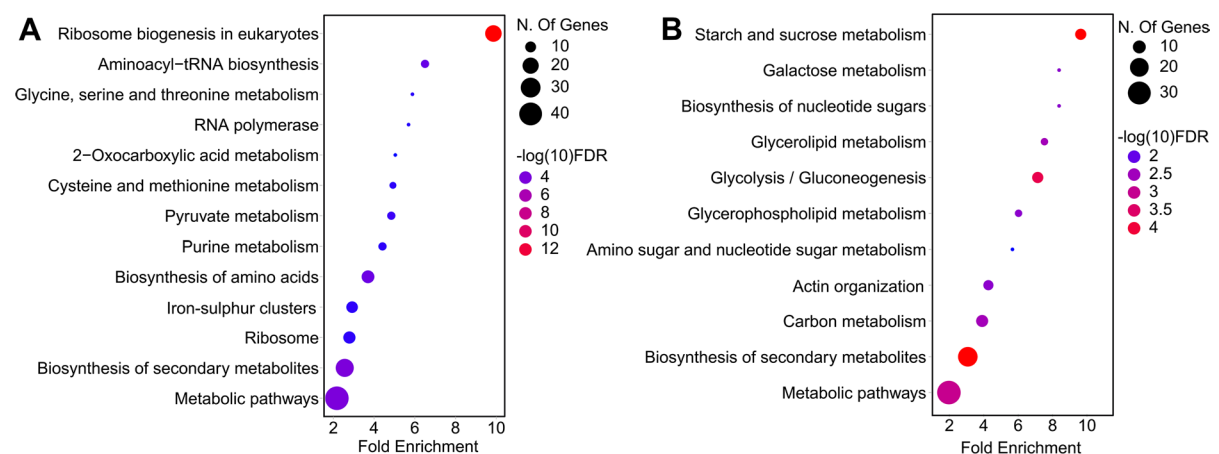
Fig. 5 Functional enrichment of proteins associated with RLS across mtKO strains. Kyoto Encyclopedia of Genes and Genomes (KEGG) pathway enrichment analyses were con-
