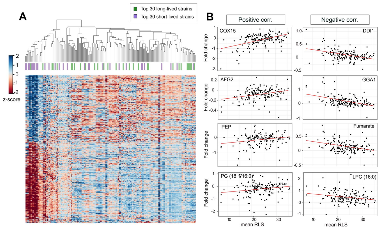
Fig. 4 Selected endophenotypes correlating with mean RLS. A ) The heat map on the left panel shows expression patterns of the significantly correlating proteins. Spearman correlation matrix of aggregated protein expression profiles across strains was used for clustering. The top 30 short- and long-lived
