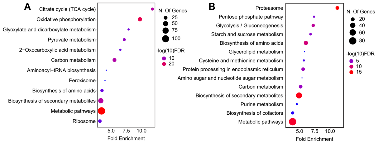
Fig. 3 Functional enrichment of proteins associated with CLS across mtKO strains. Kyoto Encyclopedia of Genes and Genomes (KEGG) pathway enrichment analyses were con-
