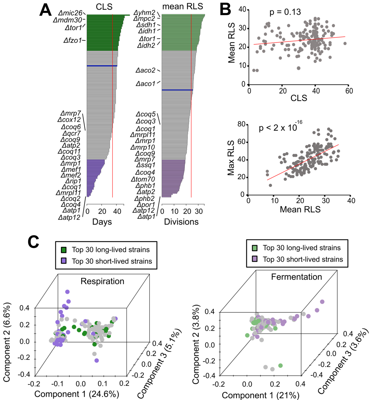
Fig. 1 Phenotypic variation across mtKO strains. A ) CLS and mean RLS variation. Green and purple bars show top long- and short-lived strains, respectively. Blue bars indicate the lifespan of the WT control. Vertical red lines depict the average CLS (34 days) and mean RLS (24 divisions) across mtKO strains. The mean and maximum RLS values and CLS phenotype of mtKO strains can be found in Supplementary Table 1. Raw RLS values can be obtained from the previously pub-
