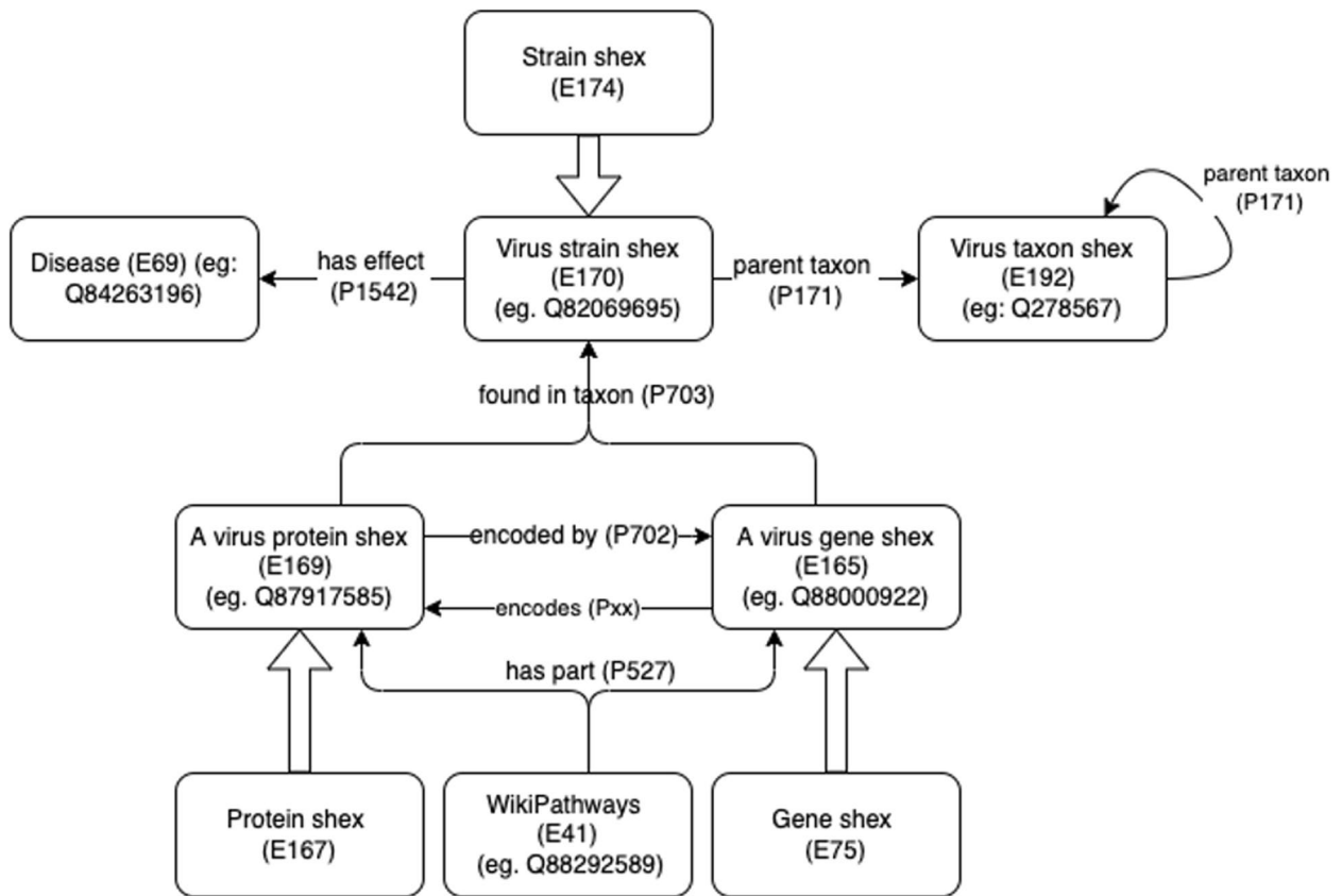
Fig. 3 Overview of the ShEx schemas and the relations between them. All shapes, properties, and items are available from within Wikidata
