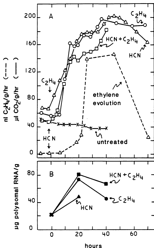
FIG. 7. A, effect of 10 \mu\text{l/l} ethylene and/or 500 \mu\text{l/l} cyanide on respiration of avocado fruit, and the effect of 500 \mu\text{l/l} cyanide on the endogenous synthesis of ethylene in avocado fruit. B, effect of 10 \mu\text{l/l} ethylene and/or 500 \mu\text{l/l} cyanide on polysome prevalence in avocado fruit. (X), untreated fruit; ( \Delta , \blacktriangle ), HCN; ( \square , \blacksquare ), HCN and \text{C}_2\text{H}_4 ; ( \circ , \bullet ), \text{C}_2\text{H}_4 .
