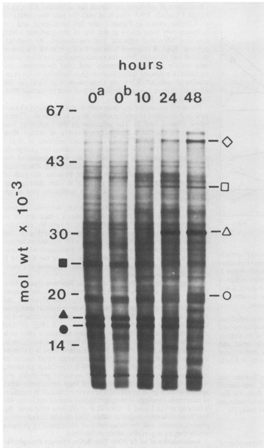
FIG. 3. Fluorograph of electrophoretically separated in vitro translation products of avocado fruit polysomal poly(A) + RNA. The number above each lane refers to hours of ethylene treatment. 0 a and 0 b refer to translation products of mRNA extracted from untreated fruit 24 and 72 h, respectively, after detaching fruit from the tree. Symbols refer to selected translation products which change in relative abundance with time. Decreasing with time: (■), 25 kD; (▲), 18 kD; (●), 17 kD. Increasing with times: (◇), 53 kD; (□), 40 kD; (△), 31 kD; (○), 20 kD.
