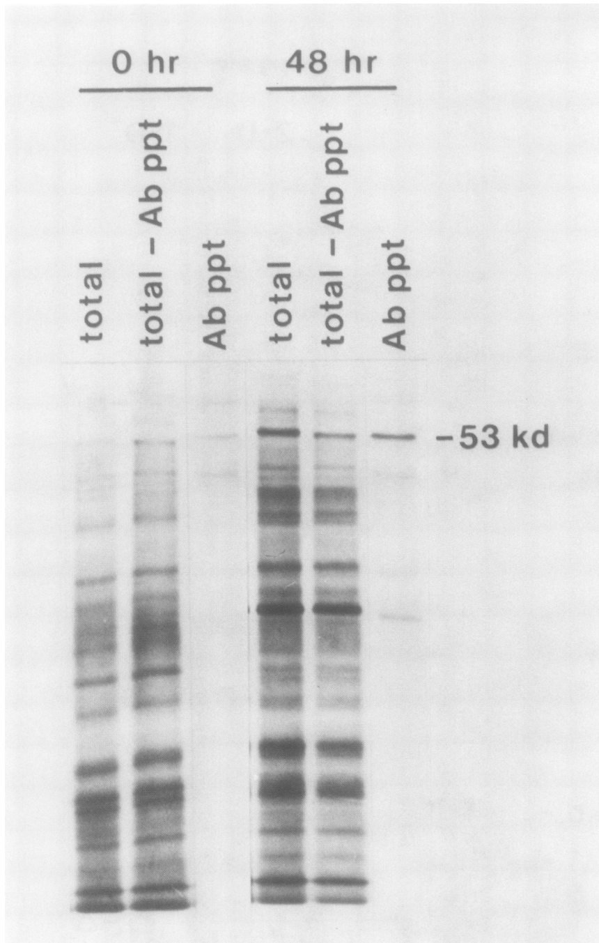
FIG. 6. Fluorograph showing immunoprecipitation of a 53-kD in vitro translation product of polysomal poly(A) + mRNA from ethylene-treated avocado fruit using avocado cellulase antiserum. Hours refer to hours of ethylene treatment. Total, total in vitro translation products; Total—Ab ppt, total minus immunoprecipitated polypeptides; Ab ppt, polypeptides which were immunoprecipitated and subsequently released.
