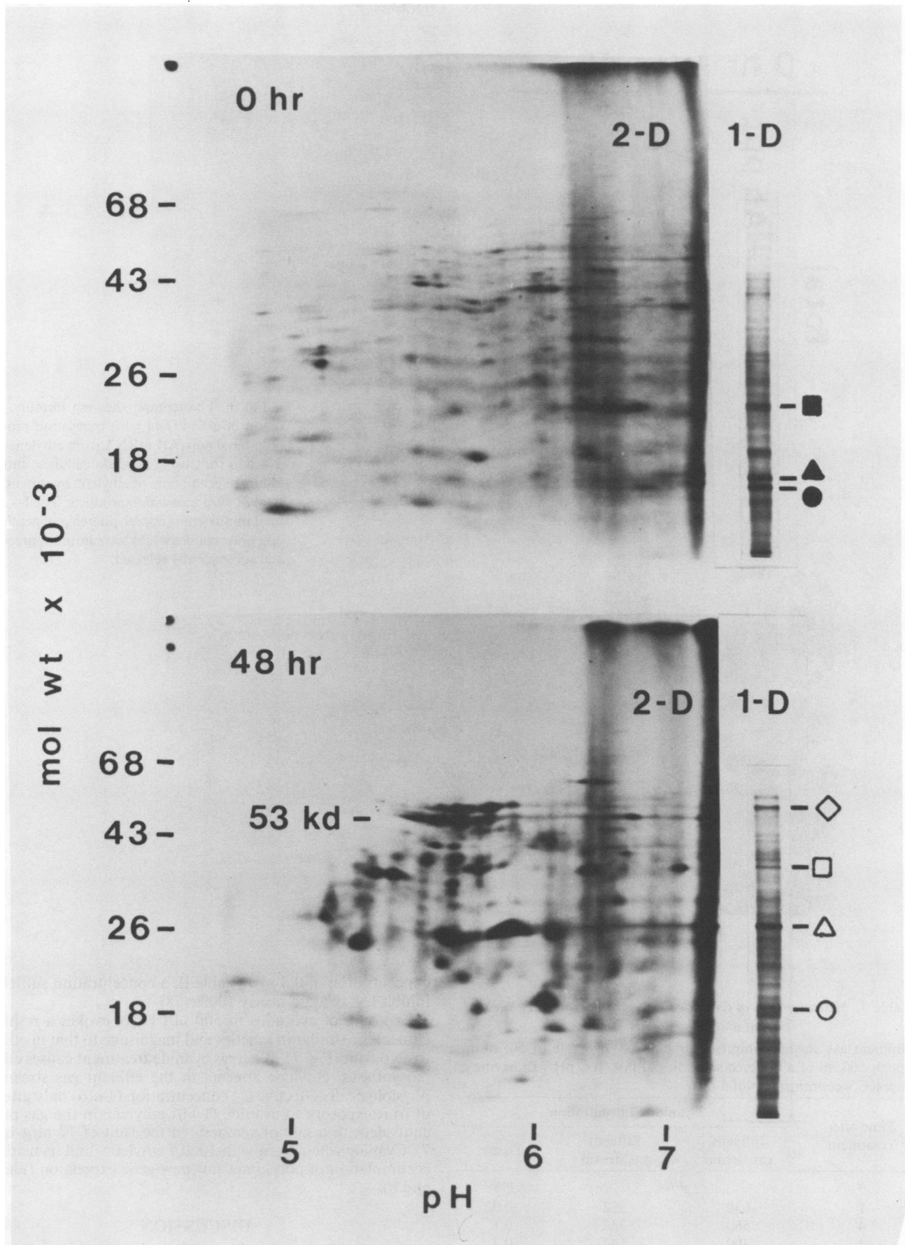
FIG. 5. Fluorograph of two-dimensional (2-D) and one-dimensional (1-D) gel electrophoresis of in vitro translation products of polysomal poly(A) + RNA extracted from untreated (0 h) avocado fruit and fruit treated with ethylene for 48 h. Symbols refer to selected in vitro translation products which change with ethylene treatment as shown in Figure 3.
