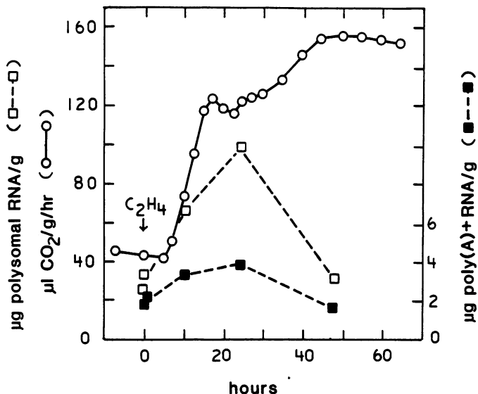
FIG. 1. Effect of 10 μl/l ethylene treatment of avocado fruit on respiration, polysome prevalence, and poly(A) + RNA extracted from polysomes. CO 2 curve is an average of three separate samples. All fruit were picked and kept at 25°C in a continuous flow of water-saturated air for 24 h prior to treatment with ethylene. Individual fruits were homogenized and RNA extracted after 0, 10, 24, and 48 h of ethylene treatment. The two 0-h samples shown for RNA quantification were homogenized for RNA extraction 24 and 72 h, respectively, after detachment from the tree.
