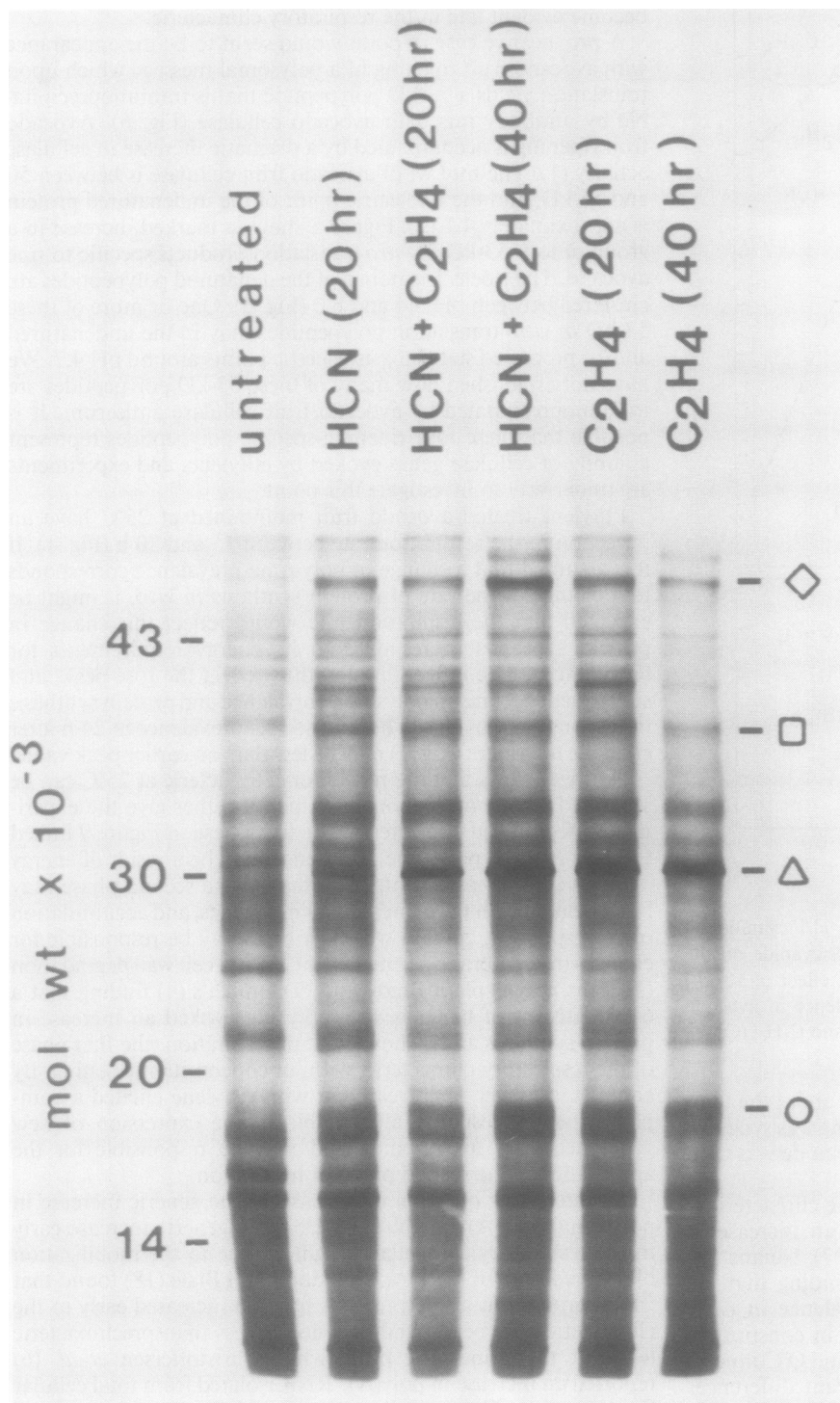
FIG. 8. Fluorograph of electrophoretically separated in vitro translation products of poly(A) + RNA from avocado fruit treated with ethylene and/or cyanide. Hours refer to hours of exposure to indicated treatments. Symbols as per Figure 3.
