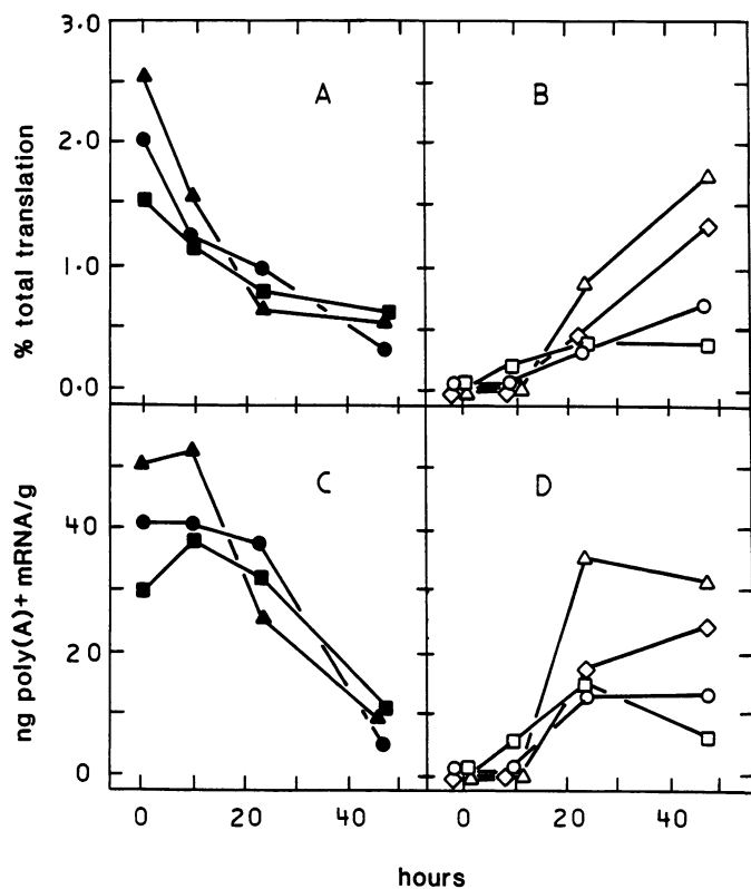
FIG. 4. Temporal change in relative abundance of poly(A) + mRNAs coding for polypeptide(s) of a specific mol wt in an in vitro translation assay. Symbols refer to in vitro translation products shown in Figure 3. A and B show percentage of relative abundance of specific messages as determined by a densitometry scan of the fluorograph in Figure 3. C and D show absolute amount of specific messages/g tissue calculated by multiplying relative abundance by \mu\text{g poly(A)}^+ RNA/g tissue.
