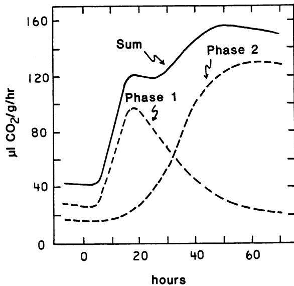
FIG. 9. Hypothesized separation of the respiratory climacteric of avocado fruit into two separate respiratory phases. Curves for phases 1 and 2 add together to give the sum curve which approximates the observed respiratory curve in Figure 1. Respiratory curve for phase 1 corresponds with the change in polysomal RNA in Figure 1.
