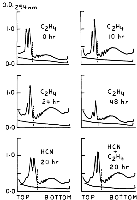
FIG. 2. Effect of 10 μl/l ethylene and/or 500 μl/l cyanide on polysome profiles of avocado fruit. Hours refer to hours of exposure to ethylene and/or cyanide. RNA associated with peaks to the left of the dashed lines were excluded from calculations for polysome prevalence in Figures 1 and 7.
