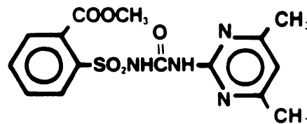
Sulfometuron Methyl
