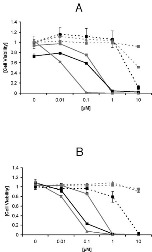
FIG. 4. Toxicities of CPT1, XF70, and XF73 for NHEKs and NHDFs after 5 min of incubation. NHEKs (A) and NHDFs (B) were incubated with different concentrations (0, 0.01, 0.1, 1.0, or 10 \mu\text{M} ) of CPT1, XF70, and XF73 for 5 min. After illumination (15.2 \text{mW}/\text{cm}^2 ; 13.7 \text{J}/\text{cm}^2 ), the cells were incubated for 24 h in the dark. Phototoxicity was tested by the standard MTT assay. Cell viability was normalized to 1; that is, the values for control cells without illumination were 1. Black line, CPT1 with illumination; gray line and \blacktriangle , XF70 with illumination; gray line and \blacktriangle , XF73 with illumination; black dotted line, CPT1 without illumination; gray dotted line and \blacktriangle , XF70 without illumination; gray dotted line and \blacktriangle , XF73 without illumination. Values are the means and standard deviations of three experiments ( P < 0.001 ).
