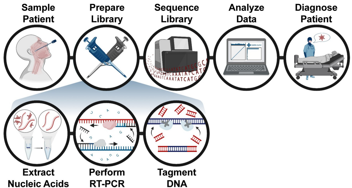
Fig 1. Pathogen-oriented low-cost assembly & re-sequencing method overview. The patient is sampled in the clinic, and the total RNA from this sample is extracted and reverse-transcribed into DNA. The sample is then enriched for SARS-CoV-2 sequence using a SARS-CoV-2 specific primer library. The amplicons then undergo a rapid tagmentation-mediated library preparation. Data is then analyzed and used to report patient results the next day.
