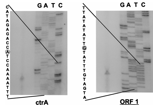
FIG. 3. Autoradiographs showing primer extension products for the serogroup A meningococcal genes ctrA and ORF1. Primer extension reactions were loaded alongside standard double-stranded DNA-sequencing reactions (load orientation of G, A, T, C) obtained by sequencing ctrA and ORF1 control DNA templates with the extension primers SE40 ( ctrA ) and SE41 (ORF1). The DNA sequence surrounding the primer extension bands has been expanded. The nucleotides corresponding to the putative start points of transcription are circled.
