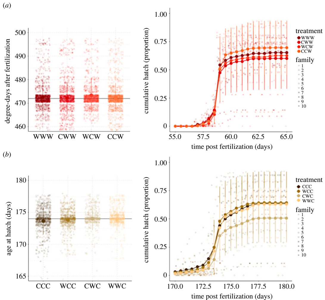
Figure 2. Age at hatching (left) and cumulative proportions of successfully hatched larvae (right) following the different combinations of gamete incubation regimes (cold (C), 2°C; warm (W), 8°C) in batches developing in the (a) warm (8°C) or (b) cold (2°C) embryo development treatment. Letters in the treatment acronyms are ordered as follows: egg temperature, sperm temperature, embryo development temperature. The means (dots) \pm standard deviations (vertical bars) are shown for a total of 80 split-design crosses, with ten males and ten females crossed pairwise in an equal number of unique families.
