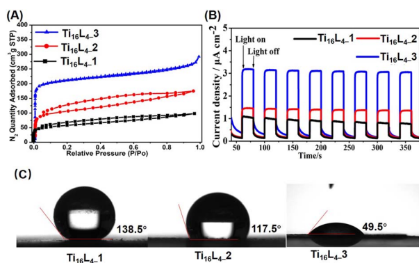
Fig. 3 (A) N 2 adsorption/desorption isotherm recorded at 77 K; (B) transient photocurrent responses of Ti 16 L 4 captured during Xe lamp irradiation in a 0.2 M Na 2 SO 4 electrolyte solution; (C) comparative assessment of the wettabilities across Ti 16 L 4-1 , Ti 16 L 4-2 and Ti 16 L 4-3 .
