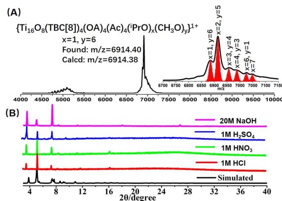
Fig. 4 (A) Positive-mode MALDI-TOF-MS spectrum depicting Ti 16 L 4-1 in CHCl 3 solution; (B) PXRD patterns of Ti 16 L 4-1 acquired during acid- and base-stability assessments. Remarkably, Ti 16 L 4-1 exhibits robustness even after prolonged exposure to 1 M HCl, HNO 3 , H 2 SO 4 , and 20 M NaOH for 24 hours.
