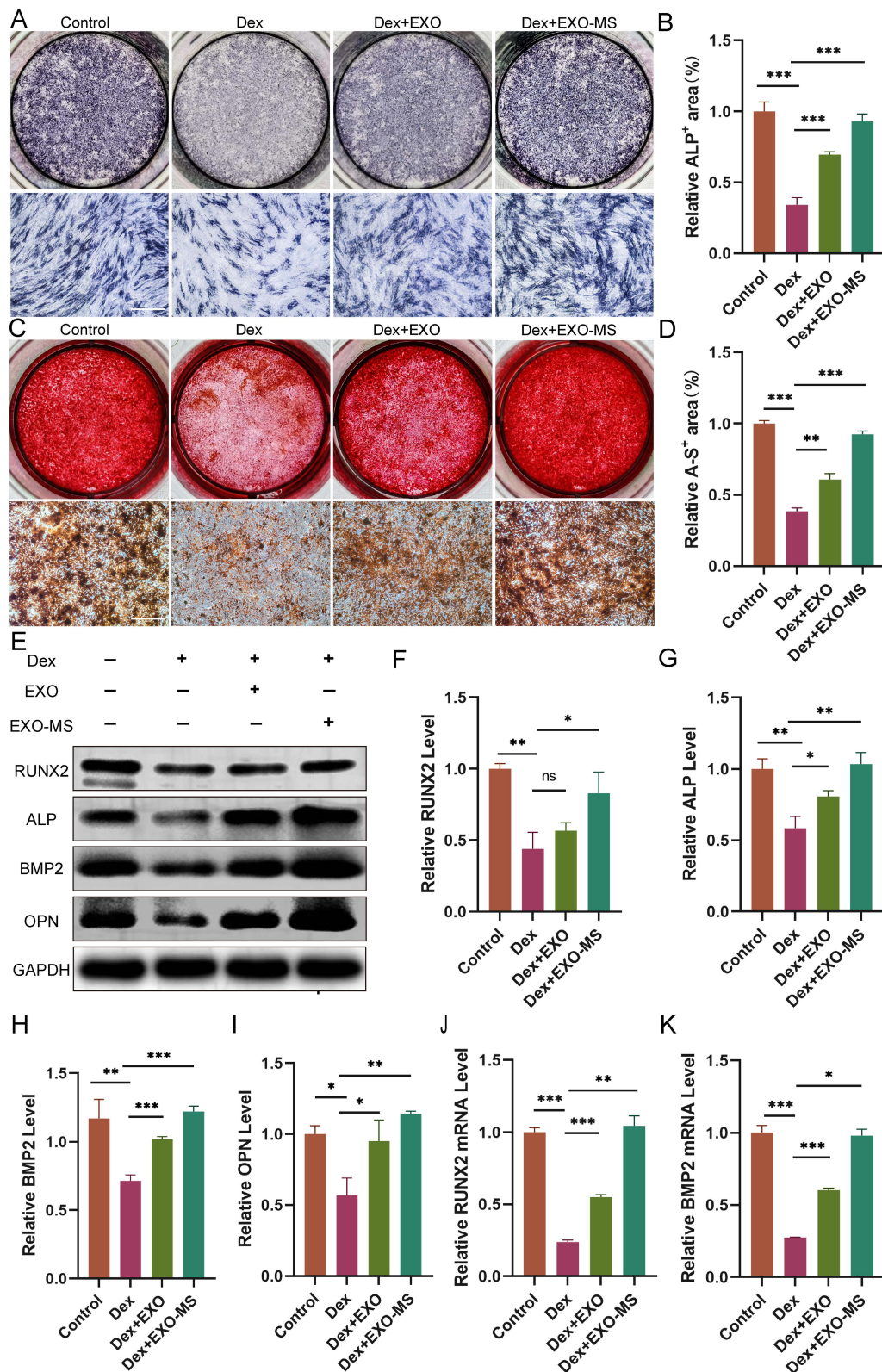
Figure 3 Effect of Exosome-MS on osteogenic differentiation of BMSCs. (A) Alkaline phosphatase (ALP) was conducted in various treatment groups (scale bar = 100 μm). (B) The statistical analysis was performed to quantify the area of ALP staining. (n=3) (C) Alizarin red staining was conducted in various treatment groups (scale bar = 100 μm). (D) The statistical analysis was performed to quantify the area of Alizarin red staining. (n=3) (E) Under the condition of dexamethasone induction, the impact of Exosome-MS on the expression levels of Runx2, ALP, BMP2, and OPN in BMSCs was determined by Western blotting. (F–I) Relative quantification of Runx2, ALP, BMP2, and OPN expression levels was carried out. (n=3) (J–K) Real-time PCR was used to confirm the expression levels of BMP2 and Runx2 in different experimental groups. The data are expressed as the mean ± SD (n = 3); *p < 0.05; **p < 0.01; ***p < 0.001.
