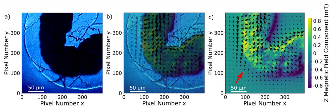
Fig. 7 (a) Transmission light microscopy image of the inset marked in a red square in Fig. 4; (b) merging of the transmission light microscopy image with the magnetic field map in (c); (c) magnetic field map, the arrows indicate the x - y component and the color bar the z -component. The bias field was subtracted for all components. The bias field direction is indicated by the red arrow.
