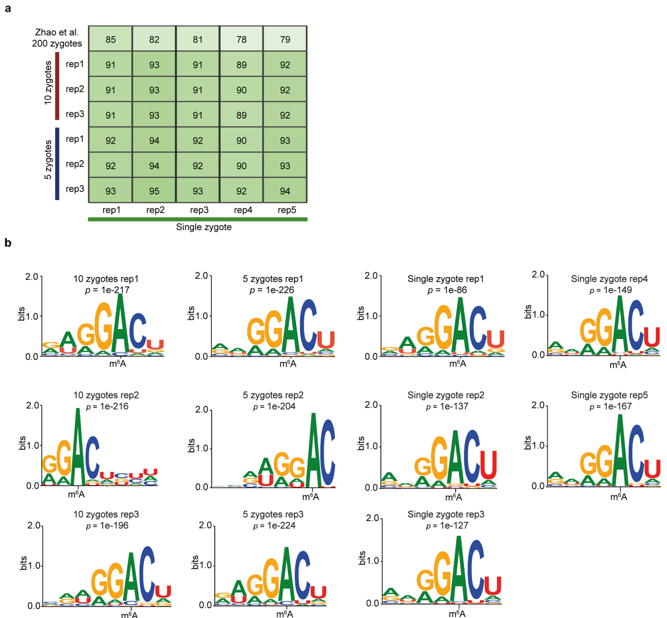
Extended Data Fig. 6 | Comparison of picoMeRIP-seq from single zebrafish zygotes and from pools of zygotes. a , Fraction of overlap of m 6 A peaks between single-zygote picoMeRIP-seq experiments and picoMeRIP-seq from pools of zygotes. The topmost row is the fraction of overlap of m 6 A transcripts
