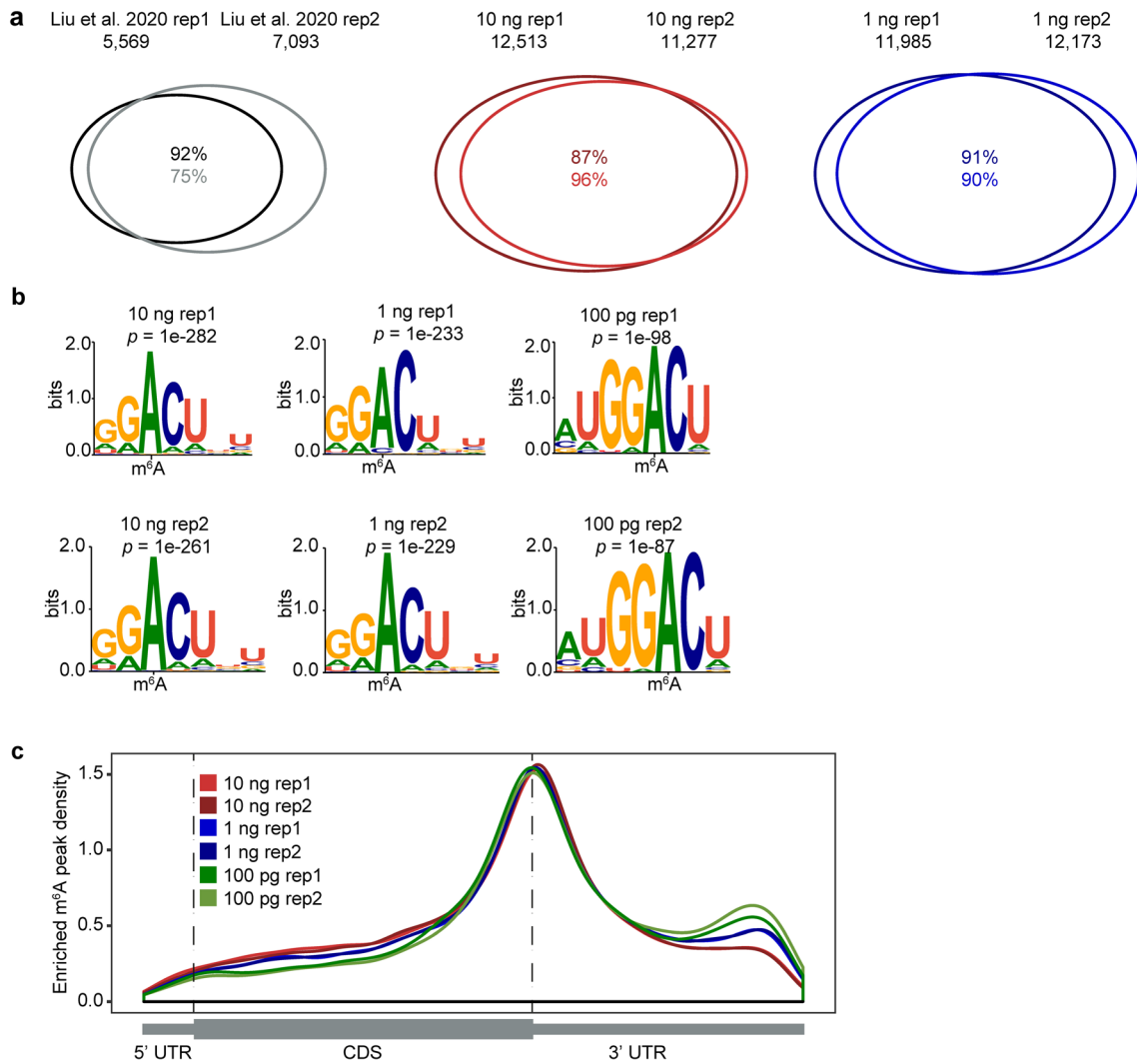
Extended Data Fig. 2 | Assessment of picoMeRIP-seq using mouse liver RNA. a , Venn diagrams showing overlap of m 6 A peaks from two replicates of published work starting with 3 \mu g total RNA (Liu et al 27 ), and for two replicates of picoMeRIP-seq experiments starting with either 10 ng or 1 ng of polyA RNA. b , Consensus
