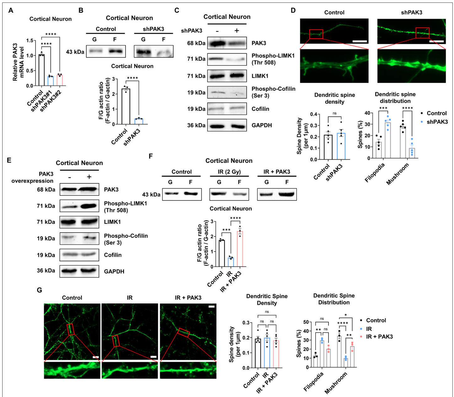
Figure 3. p21-activated kinase 3 (PAK3) regulates filamentous/globular (F/G)-actin and dendritic spine in neuron. (A) The changes of PAK3 mRNA levels after PAK3 downregulation (shPAK3) in cortical neuron. (B) The F/G-actin ratio after expression of PAK3 downregulation (shPAK3) in cortical neuron. Each filamentous actin (F-actin) and globular (G)-actin are quantified by ImageJ. (C) The protein levels of phosphorylated LIMK1, LIM kinase 1 (LIMK1), phosphorylated cofilin, and cofilin after PAK3 downregulation (shPAK3) in cortical neuron. (D) Upper: representative fluorescence image of filamentous actin (F-actin, green) after PAK3 downregulation (shPAK3) in cortical neuron. Lower: the density and distribution of dendritic spine in shPAK3 group compared to control group. Scale bars, 10 \mu m. (E) The protein levels of PAK3, phosphorylated LIMK1, LIMK1, phosphorylated cofilin, and cofilin after PAK3 overexpression in cortical neuron. (F) The F/G-actin ratio after ionizing radiation (IR) or IR with PAK3 overexpression in cortical neuron. Each F-actin and G-actin are quantified by ImageJ. (G) Upper: representative fluorescence image of filamentous actin (F-actin, green) after IR and/or PAK3 overexpression in cortical neuron. Lower: the density and distribution of dendritic spine in control, IR and/or PAK3 overexpression group. Scale bars, 10 \mu m. Statistical analysis was performed with Student's t-test for (B and D) and one-way ANOVA plus a Tukey's multiple comparisons test for (A, D, F, and G) ns, non-significant; * p < 0.05 ; ** p < 0.01 ; *** p < 0.001 ; **** p < 0.0001 .
