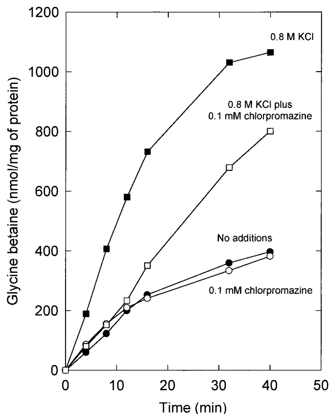
FIG. 5. Effect of chlorpromazine on the uptake of [ ^{14} C]glycine betaine. Cells of L. plantarum ATCC 14917 were grown on CDM containing 0.8 M KCl, washed, and resuspended in 50 mM potassium phosphate (pH 6.5). The concentrated cell suspensions were diluted in 50 mM potassium phosphate (pH 6.5) to a final protein concentration of 0.17 mg/ml. After 6 min of preenergization with 10 mM glucose, uptake was initiated at time zero by the addition of [ ^{14} C]glycine betaine (final concentration of 1.3 mM) without (closed symbols) or with (open symbols) 0.1 mM chlorpromazine (final concentration). The uptake was assayed without (circles) or with (squares) 0.8 M KCl (final concentration) added together with the [ ^{14} C]glycine betaine.
