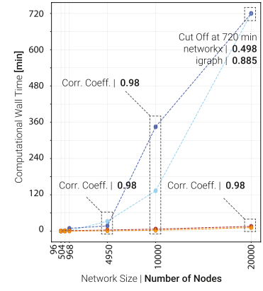
F | Wall time comparison for equal Pearson correlation coefficient
