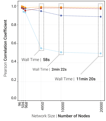
E | Pearson correlation coefficient for equal computational wall time
