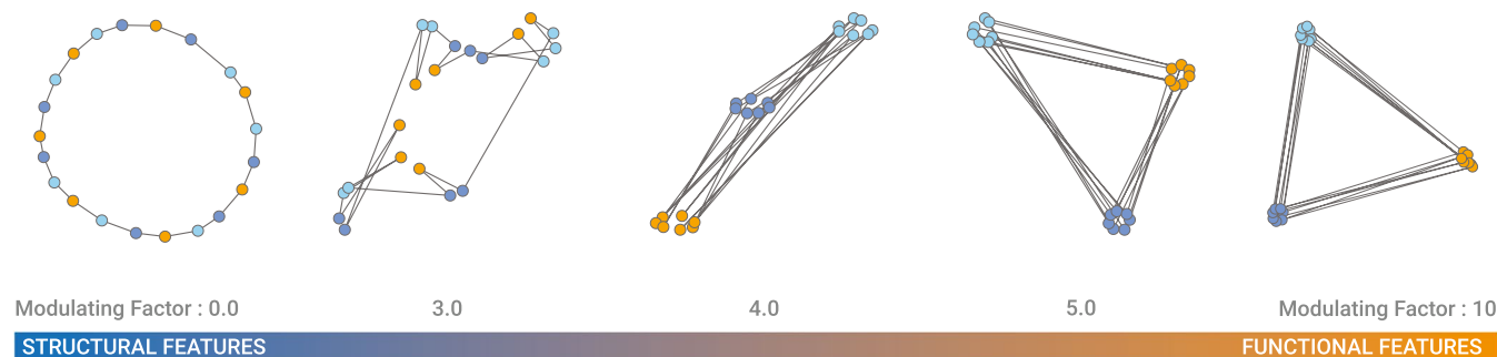
Extended Data Fig. 5 | Combined structural and functional layout. A Illustration of the method for generating layouts that combine structural and functional features in a tunable fashion. The structural aspect of the layout is derived from the global layout, where each node in the network is represented by a feature vector containing random walk visiting frequencies to all other nodes. The functional aspect is then introduced by adding an additional column for each functional feature to be included in the layout, for example associations with different diseases. These functional columns contain values '1' or '0', depending on whether a particular node is associated with the respective feature (value '1') or not (value '0'). Scaling the functional columns by a factor m \geq 0 allows to modulate between purely structural layouts ( m=0 ) and layouts that are increasingly dominated by the functional annotations ( m>0 ). B Application of the method to a simple model network with ring structure three node annotations, indicated by different colors. As the modulation factor increases from m=0 to m=10 , the layout transitions from a purely structural one, to one dominated by the node annotations alone.
