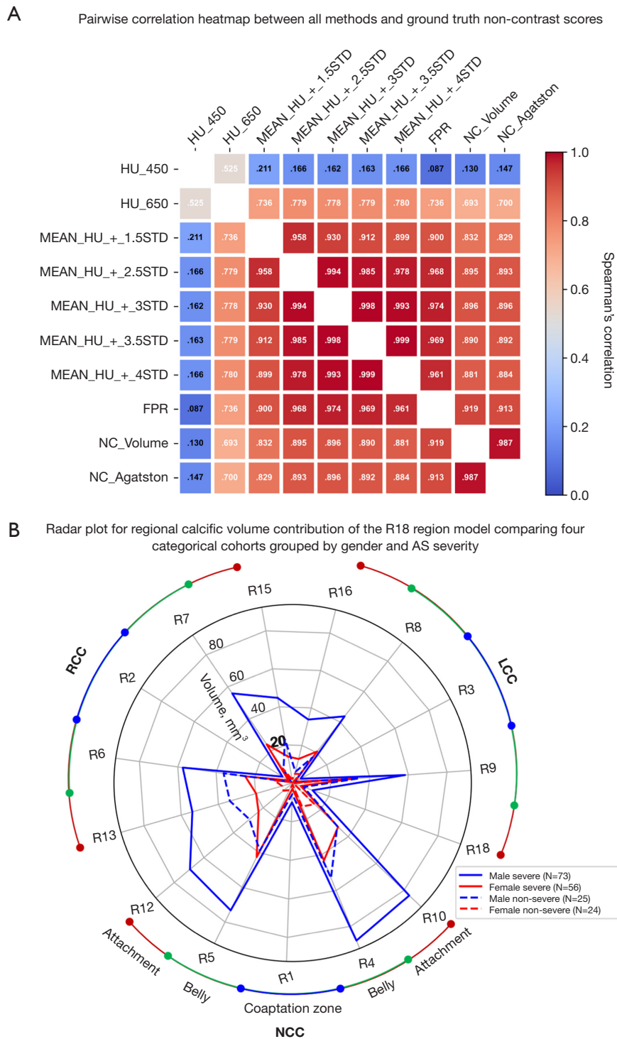
Figure 6 Comparative analysis of calcific detection methods and regional distribution of calcification across the cohort (N=178). (A) Spearman's correlation heatmap between all contrast calcific volume scores and non-contrast volume and Agatston scores. (B) Radar plot with categories grouped by sex and AS severity showing regional median volume spread in each region defined in Figure 1C . AS, aortic stenosis.
