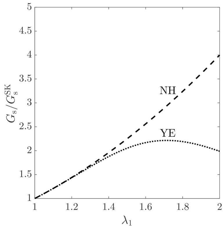
Figure 1: Variation of the shear elastic modulus G_s of the neo-Hookean (NH) and Yeoh (YE) laws, normalized with the shear elastic modulus of Skalak law ( G_s^{SK} ), with respect to the principal extension ratio \lambda_1 , so that all constitutive laws produce the same principal tension T_1 .
