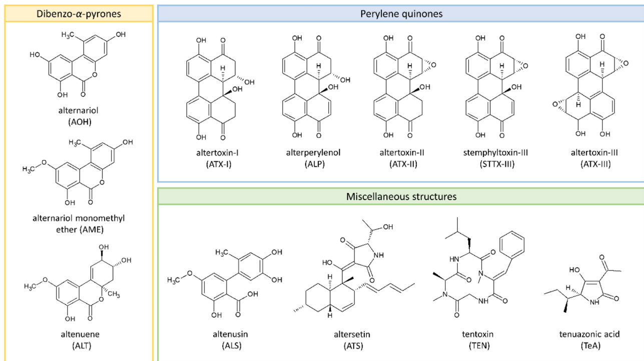
Fig. 1 The structures of Alternaria mycotoxins: alternariol (AOH), alternariol monomethyl ether (AME), altenuene (ALT), altenusin (ALS), altersetin (ATS), tentoxin (TEN) tenuazonic acid (TeA) and
