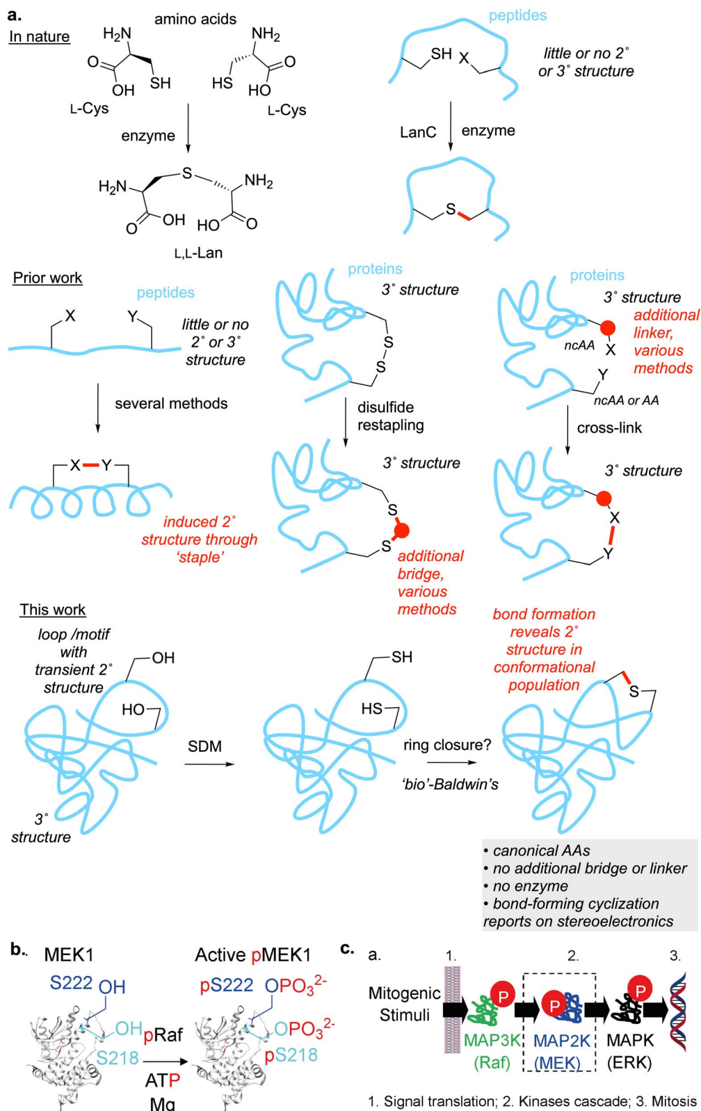
Fig. 1 Stapling in MEK1. (a) (Top) Lan is formed enzymatically between amino acids and in peptides but not proteins. (Middle) Stapling methods used in peptides can stabilize extracted motifs and large cycles can bridge some proteins, albeit often with extended bridges or linkers and/or through use of reactive, non-canonical amino acids (ncAAs) that may not be driven by reactivity that reports on conformation; SDM = site directed mutagenesis. In this work: we propose Lan as a minimal staple that might, through a set of cyclization rules, report upon conformations that enable stapling chemistries, likely in minimal motifs more likely to be under conformational control of relevance to function. (b) Enzymatic phosphorylation at sites Ser218, Ser222 in its activation loop is the primary mode of activation of MEK1. (c) The Raf-MEK-ERK MAPK signaling cascade.
