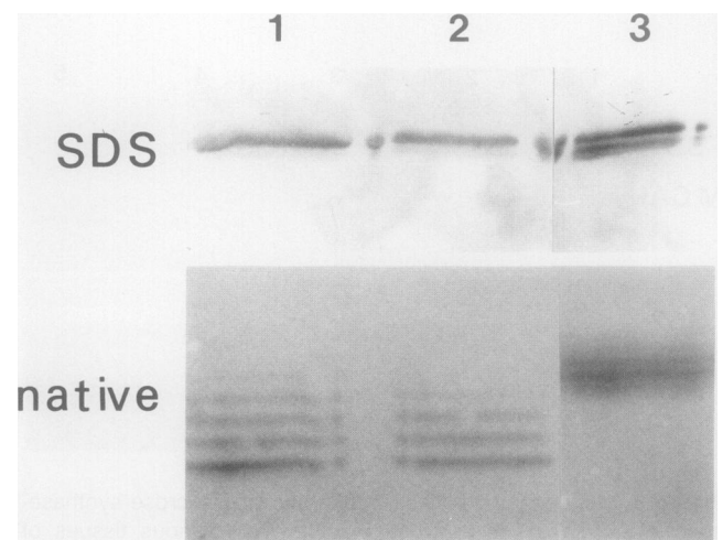
Figure 6. Denaturing (30 \mu g) and nondenaturing (60 \mu g) (as indicated) Western blots showing sucrose synthase-specific protein bands, through the maize SS1 polyclonal antibody, in seedling extracts of: lane 1, aerobic control; lane 2, anaerobic; lane 3, maize root extract (30 \mu g for either type of gel). Values in parentheses represent the amount of soluble protein.
